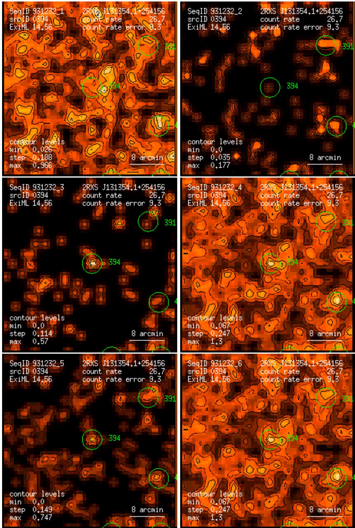
Figure 394: RASS 931232: detection 0394: band rate images, Gaussian filter: (1) PSPC channels 11 – 41, (2) 52 – 90, (3) 91 – 201, (4) 11 – 235, (5) 52 – 201, (6) 11 – 201. Broad band rates in counts/ks. Band rate contour levels in counts/ks/arcmin 2 .
