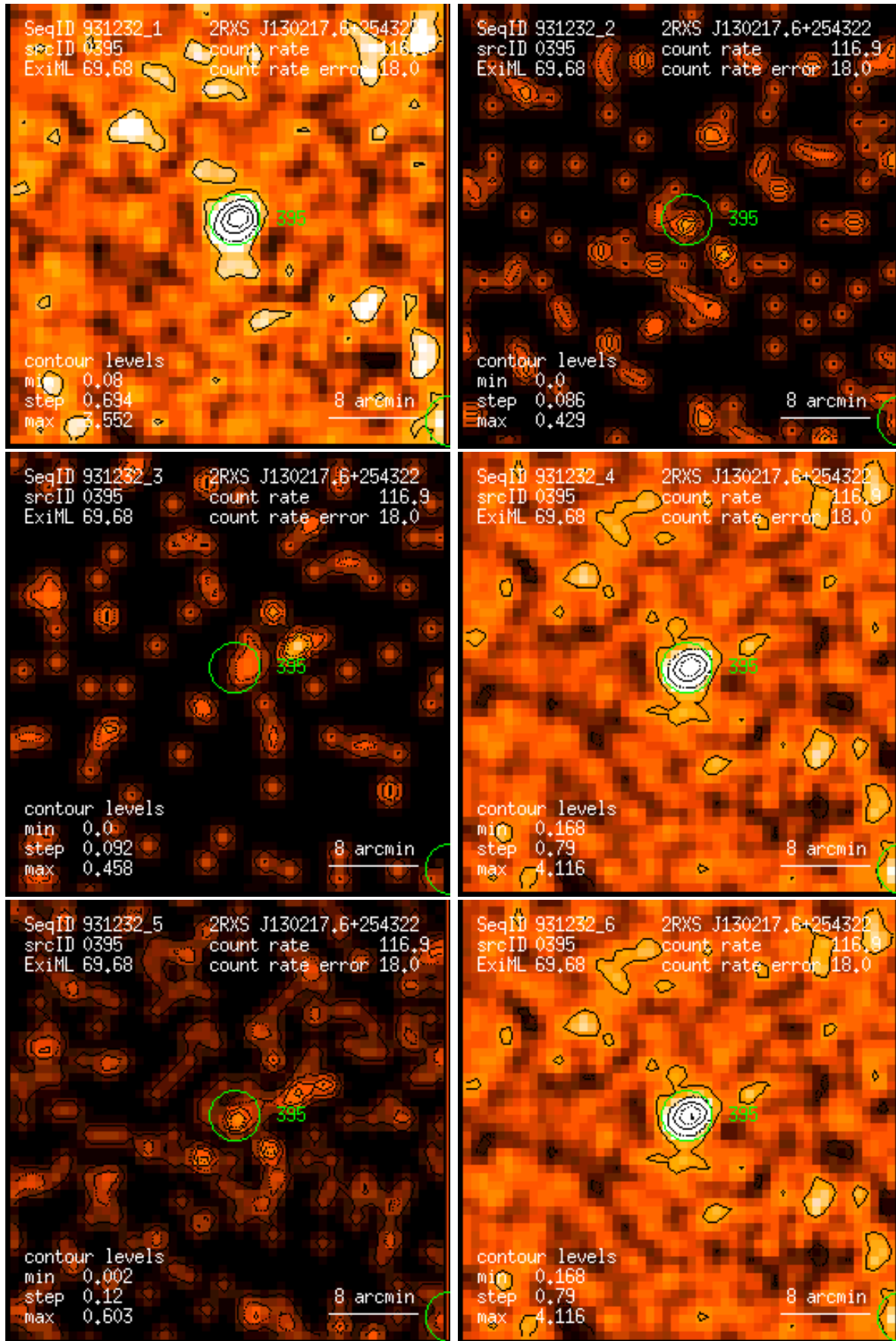
Figure 395: RASS 931232: detection 0395: band rate images, Gaussian filter: (1) PSPC channels 11 – 41, (2) 52 – 90, (3) 91 – 201, (4) 11 – 235, (5) 52 – 201, (6) 11 – 201. Broad band rates in counts/ks. Band rate contour levels in counts/ks/arcmin 2 .
