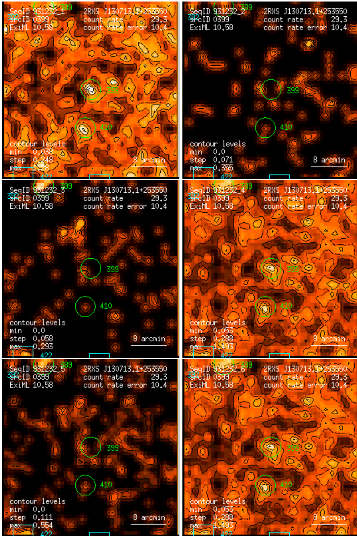
Figure 399: RASS 931232: detection 0399: band rate images, Gaussian filter: (1) PSPC channels 11 – 41, (2) 52 – 90, (3) 91 – 201, (4) 11 – 235, (5) 52 – 201, (6) 11 – 201. Broad band rates in counts/ks. Band rate contour levels in counts/ks/arcmin 2 .
