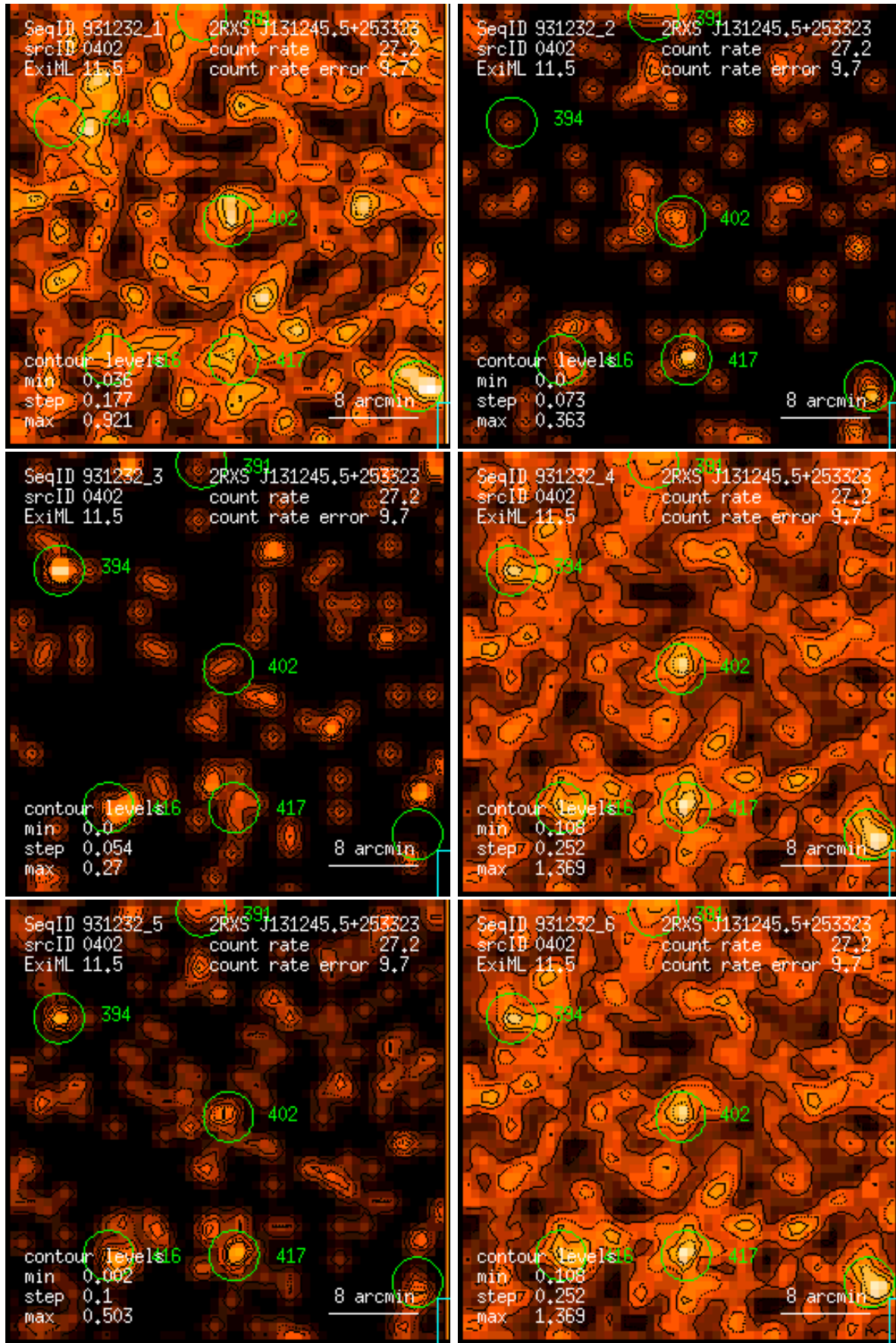
Figure 402: RASS 931232: detection 0402: band rate images, Gaussian filter: (1) PSPC channels 11 – 41, (2) 52 – 90, (3) 91 – 201, (4) 11 – 235, (5) 52 – 201, (6) 11 – 201. Broad band rates in counts/ks. Band rate contour levels in counts/ks/arcmin 2 .
