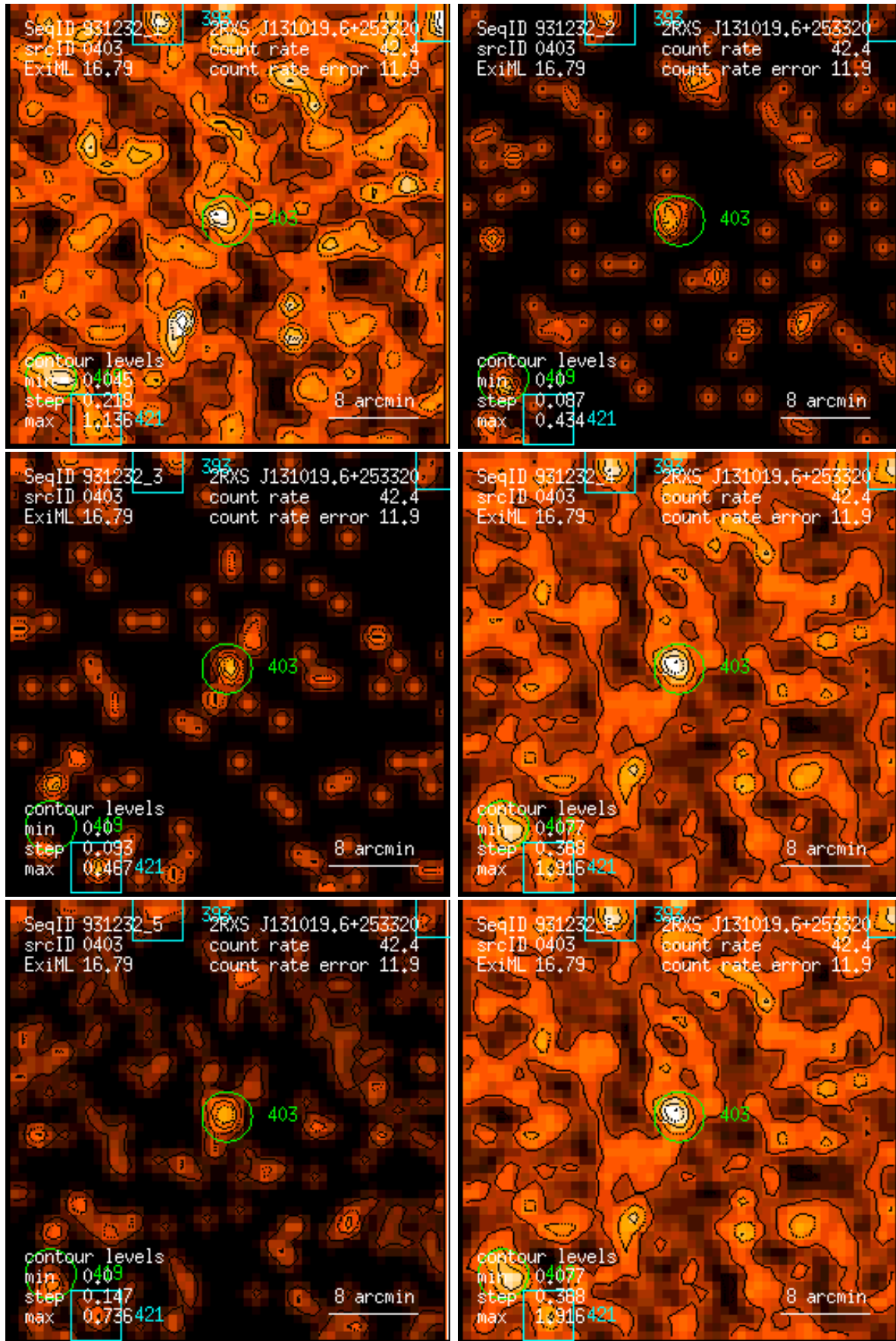
Figure 403: RASS 931232: detection 0403: band rate images, Gaussian filter: (1) PSPC channels 11 – 41, (2) 52 – 90, (3) 91 – 201, (4) 11 – 235, (5) 52 – 201, (6) 11 – 201. Broad band rates in counts/ks. Band rate contour levels in counts/ks/arcmin 2 .
