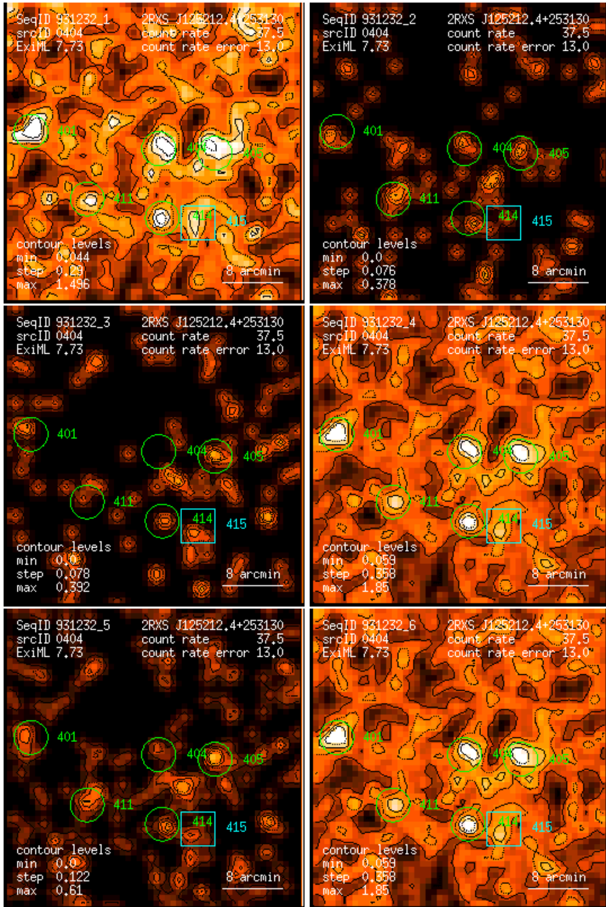
Figure 404: RASS 931232: detection 0404: band rate images, Gaussian filter: (1) PSPC channels 11 – 41, (2) 52 – 90, (3) 91 – 201, (4) 11 – 235, (5) 52 – 201, (6) 11 – 201. Broad band rates in counts/ks. Band rate contour levels in counts/ks/arcmin 2 .
