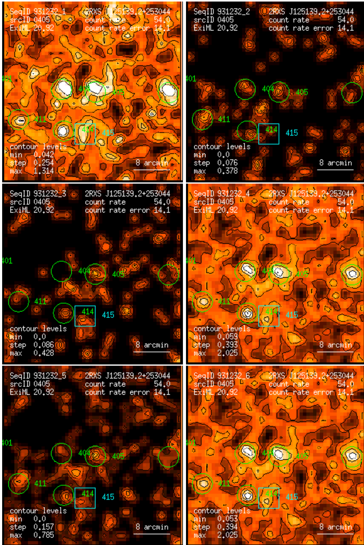
Figure 405: RASS 931232: detection 0405: band rate images, Gaussian filter: (1) PSPC channels 11 – 41, (2) 52 – 90, (3) 91 – 201, (4) 11 – 235, (5) 52 – 201, (6) 11 – 201. Broad band rates in counts/ks. Band rate contour levels in counts/ks/arcmin 2 .
