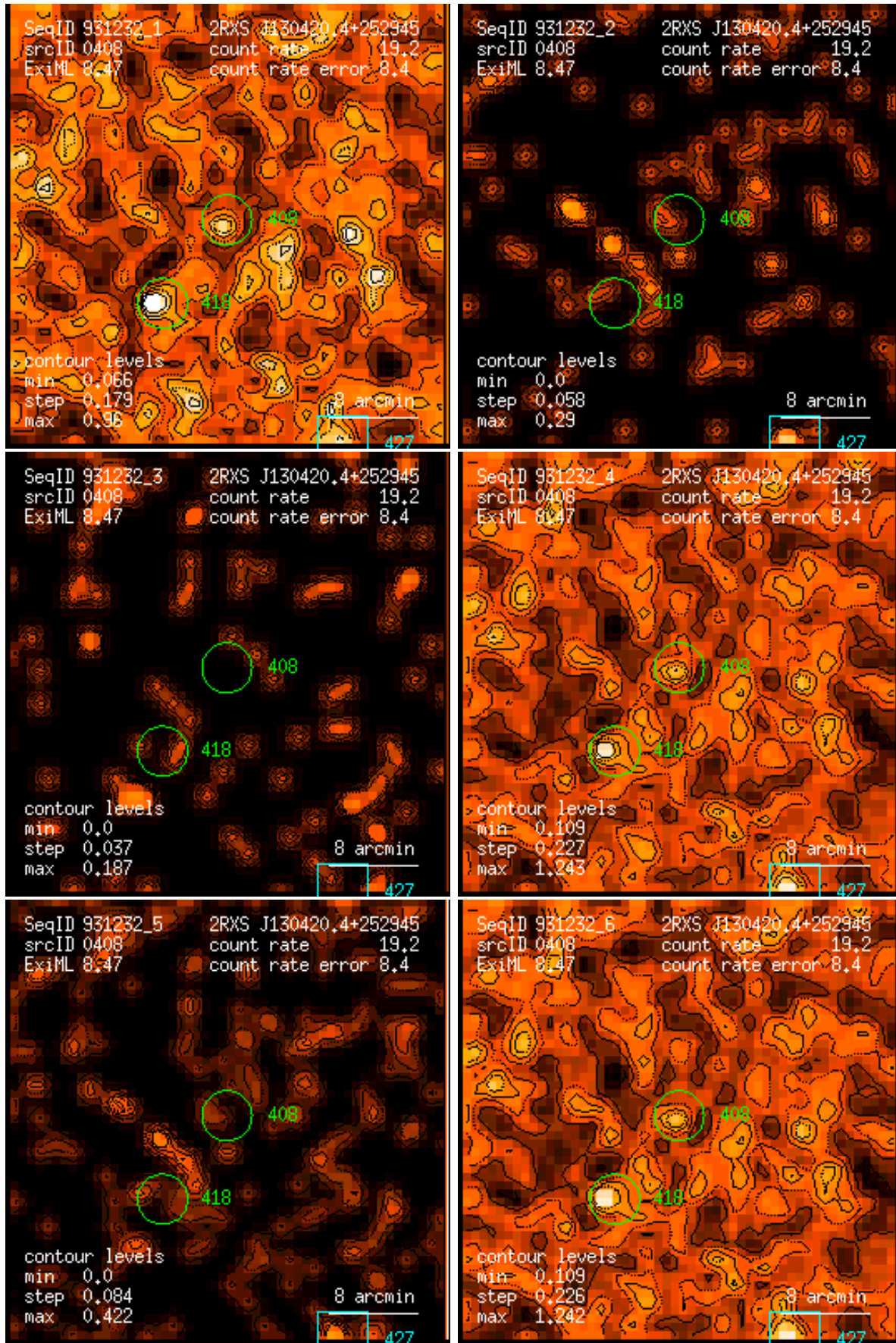
Figure 408: RASS 931232: detection 0408: band rate images, Gaussian filter: (1) PSPC channels 11 – 41, (2) 52 – 90, (3) 91 – 201, (4) 11 – 235, (5) 52 – 201, (6) 11 – 201. Broad band rates in counts/ks. Band rate contour levels in counts/ks/arcmin 2 .
