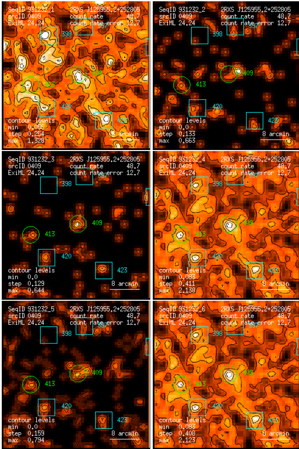
Figure 409: RASS 931232: detection 0409: band rate images, Gaussian filter: (1) PSPC channels 11 – 41, (2) 52 – 90, (3) 91 – 201, (4) 11 – 235, (5) 52 – 201, (6) 11 – 201. Broad band rates in counts/ks. Band rate contour levels in counts/ks/arcmin 2 .
