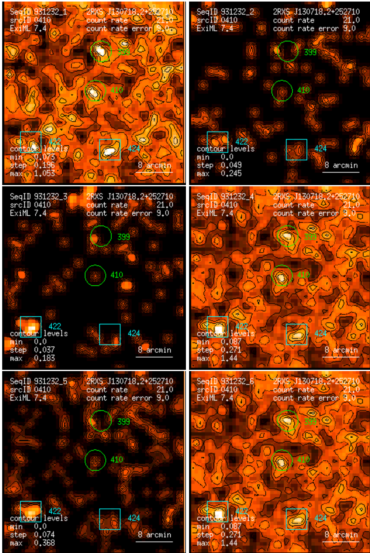
Figure 410: RASS 931232: detection 0410: band rate images, Gaussian filter: (1) PSPC channels 11 – 41, (2) 52 – 90, (3) 91 – 201, (4) 11 – 235, (5) 52 – 201, (6) 11 – 201. Broad band rates in counts/ks. Band rate contour levels in counts/ks/arcmin 2 .
