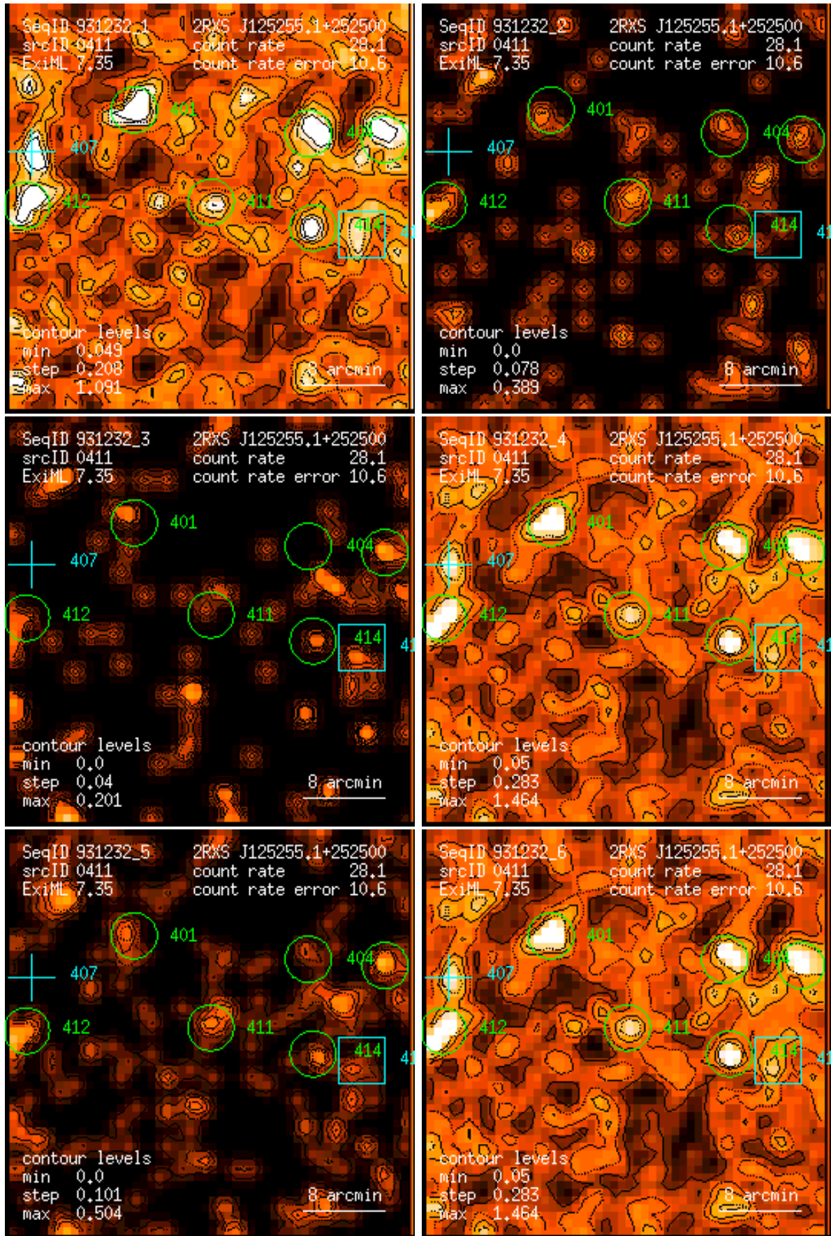
Figure 411: RASS 931232: detection 0411: band rate images, Gaussian filter: (1) PSPC channels 11 – 41, (2) 52 – 90, (3) 91 – 201, (4) 11 – 235, (5) 52 – 201, (6) 11 – 201. Broad band rates in counts/ks. Band rate contour levels in counts/ks/arcmin 2 .
