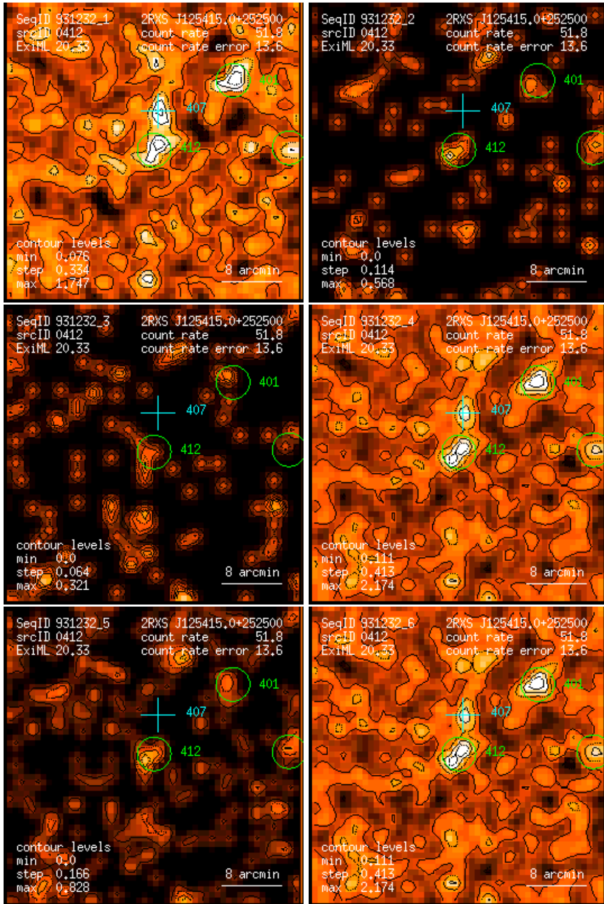
Figure 412: RASS 931232: detection 0412: band rate images, Gaussian filter: (1) PSPC channels 11 – 41, (2) 52 – 90, (3) 91 – 201, (4) 11 – 235, (5) 52 – 201, (6) 11 – 201. Broad band rates in counts/ks. Band rate contour levels in counts/ks/arcmin 2 .
