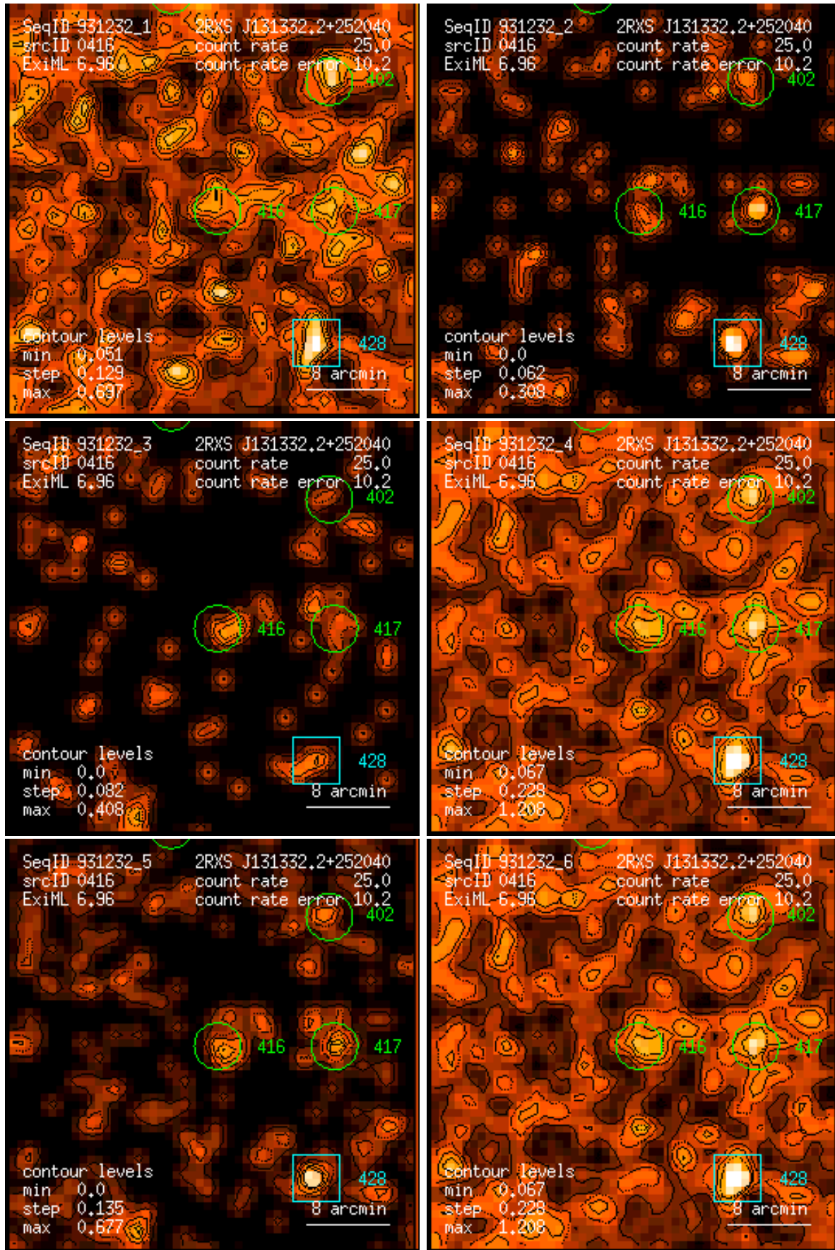
Figure 416: RASS 931232: detection 0416: band rate images, Gaussian filter: (1) PSPC channels 11 – 41, (2) 52 – 90, (3) 91 – 201, (4) 11 – 235, (5) 52 – 201, (6) 11 – 201. Broad band rates in counts/ks. Band rate contour levels in counts/ks/arcmin 2 .
