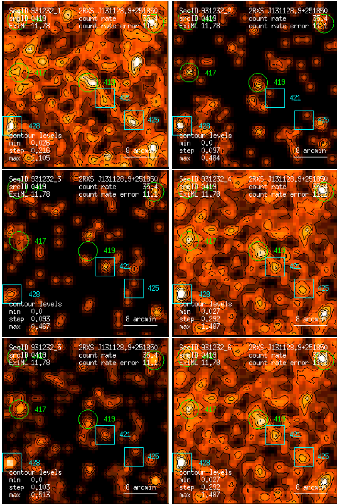
Figure 419: RASS 931232: detection 0419: band rate images, Gaussian filter: (1) PSPC channels 11 – 41, (2) 52 – 90, (3) 91 – 201, (4) 11 – 235, (5) 52 – 201, (6) 11 – 201. Broad band rates in counts/ks. Band rate contour levels in counts/ks/arcmin 2 .
