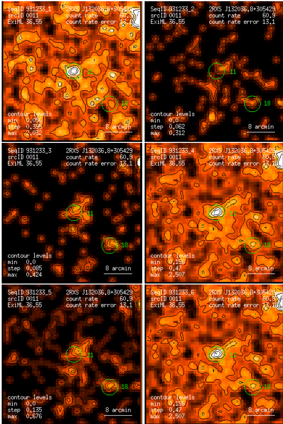
Figure 11: RASS 931233: detection 0011: band rate images, Gaussian filter: (1) PSPC channels 11 – 41, (2) 52 – 90, (3) 91 – 201, (4) 11 – 235, (5) 52 – 201, (6) 11 – 201. Broad band rates in counts/ks. Band rate contour levels in counts/ks/arcmin 2 .
