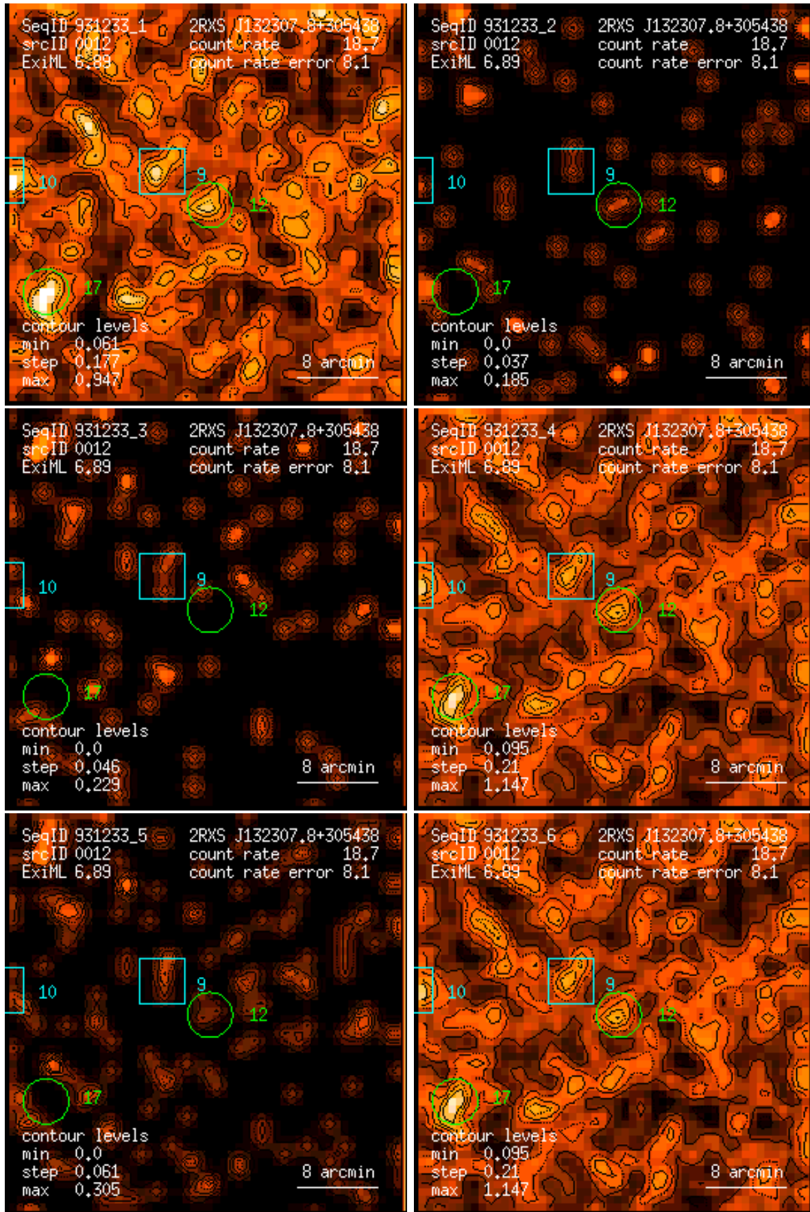
Figure 12: RASS 931233: detection 0012: band rate images, Gaussian filter: (1) PSPC channels 11 – 41, (2) 52 – 90, (3) 91 – 201, (4) 11 – 235, (5) 52 – 201, (6) 11 – 201. Broad band rates in counts/ks. Band rate contour levels in counts/ks/arcmin 2 .
