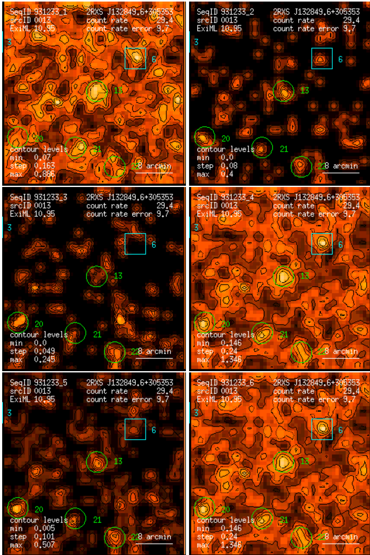
Figure 13: RASS 931233: detection 0013: band rate images, Gaussian filter: (1) PSPC channels 11 – 41, (2) 52 – 90, (3) 91 – 201, (4) 11 – 235, (5) 52 – 201, (6) 11 – 201. Broad band rates in counts/ks. Band rate contour levels in counts/ks/arcmin 2 .
