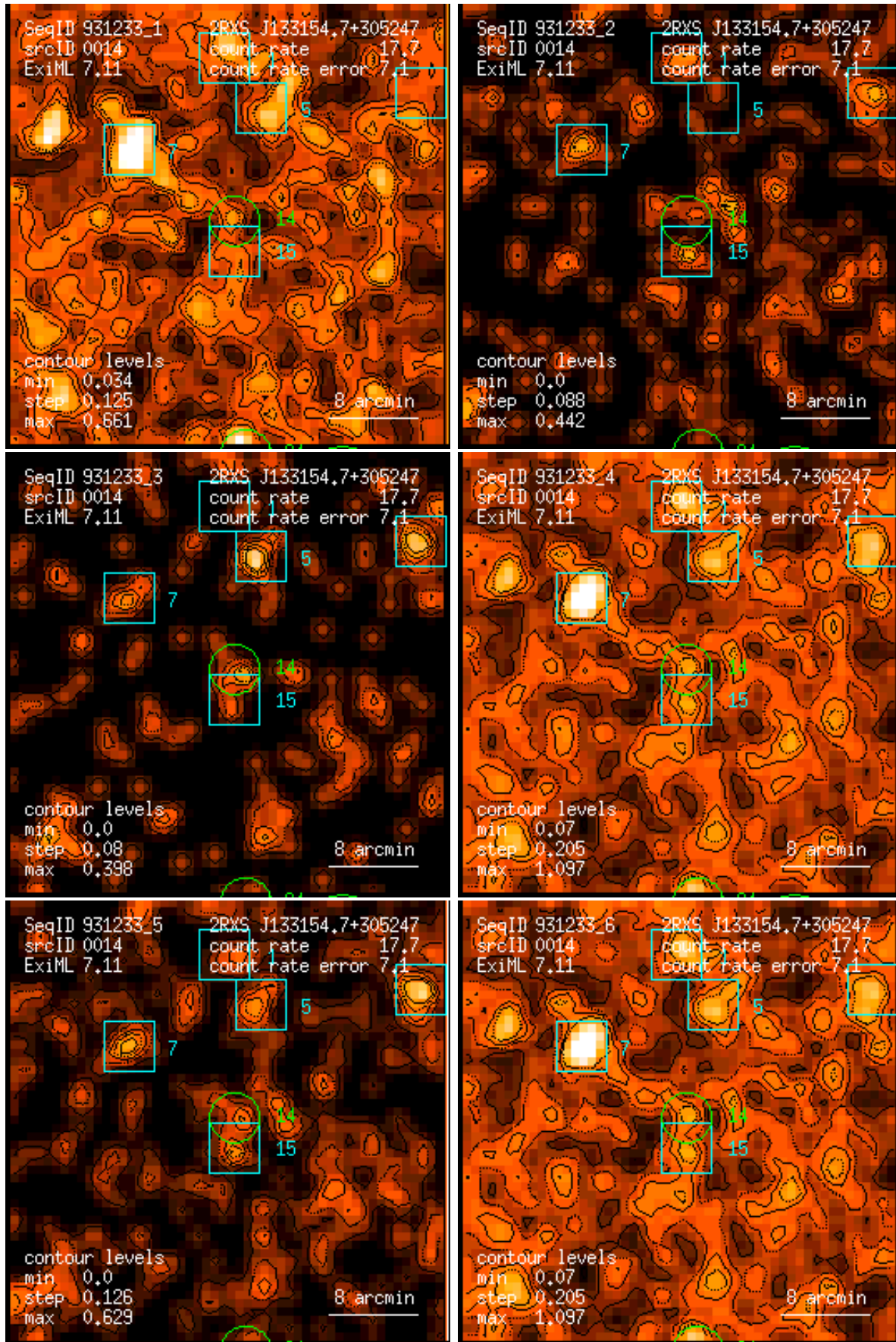
Figure 14: RASS 931233: detection 0014: band rate images, Gaussian filter: (1) PSPC channels 11 – 41, (2) 52 – 90, (3) 91 – 201, (4) 11 – 235, (5) 52 – 201, (6) 11 – 201. Broad band rates in counts/ks. Band rate contour levels in counts/ks/arcmin 2 .
