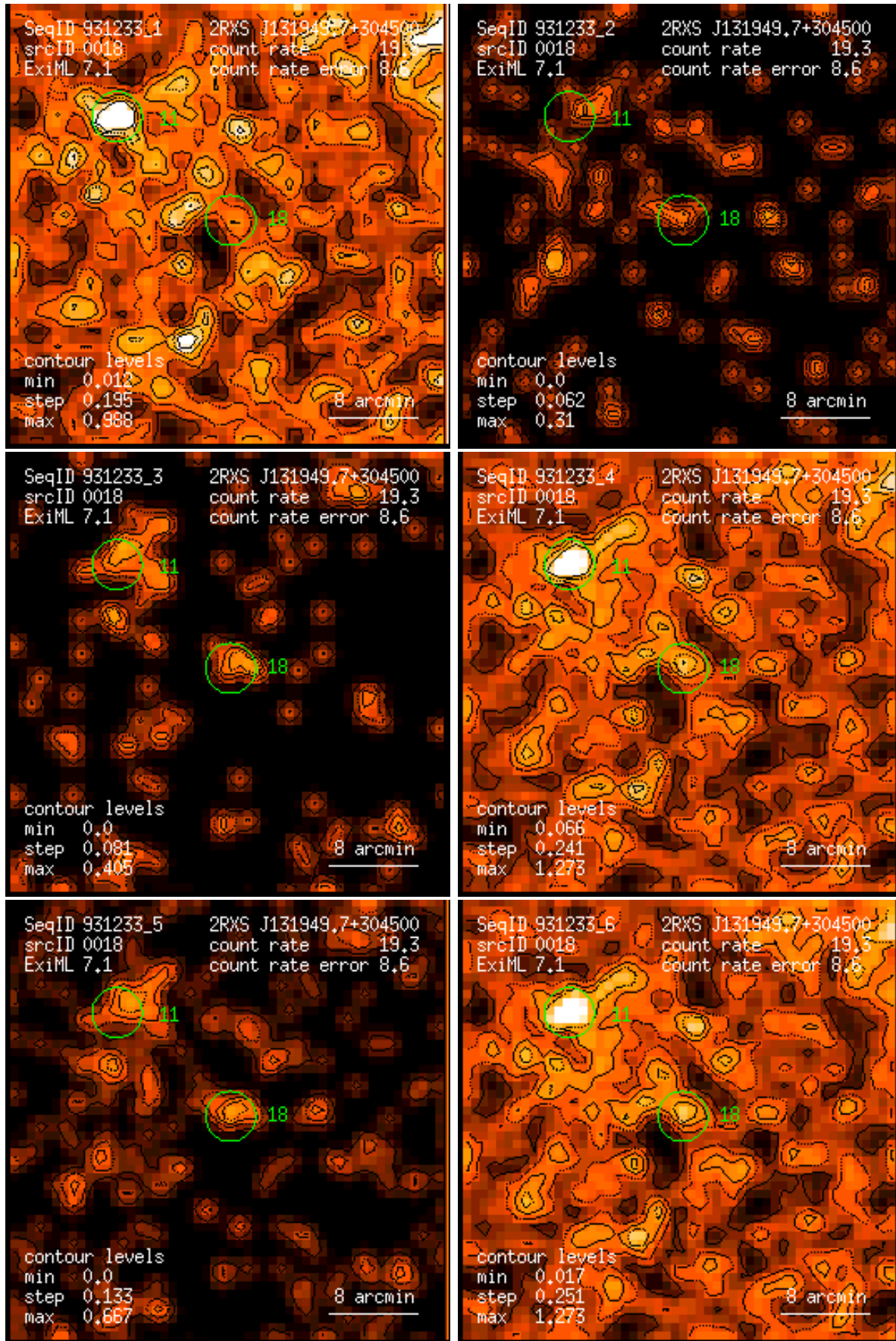
Figure 18: RASS 931233: detection 0018: band rate images, Gaussian filter: (1) PSPC channels 11 – 41, (2) 52 – 90, (3) 91 – 201, (4) 11 – 235, (5) 52 – 201, (6) 11 – 201. Broad band rates in counts/ks. Band rate contour levels in counts/ks/arcmin 2 .
