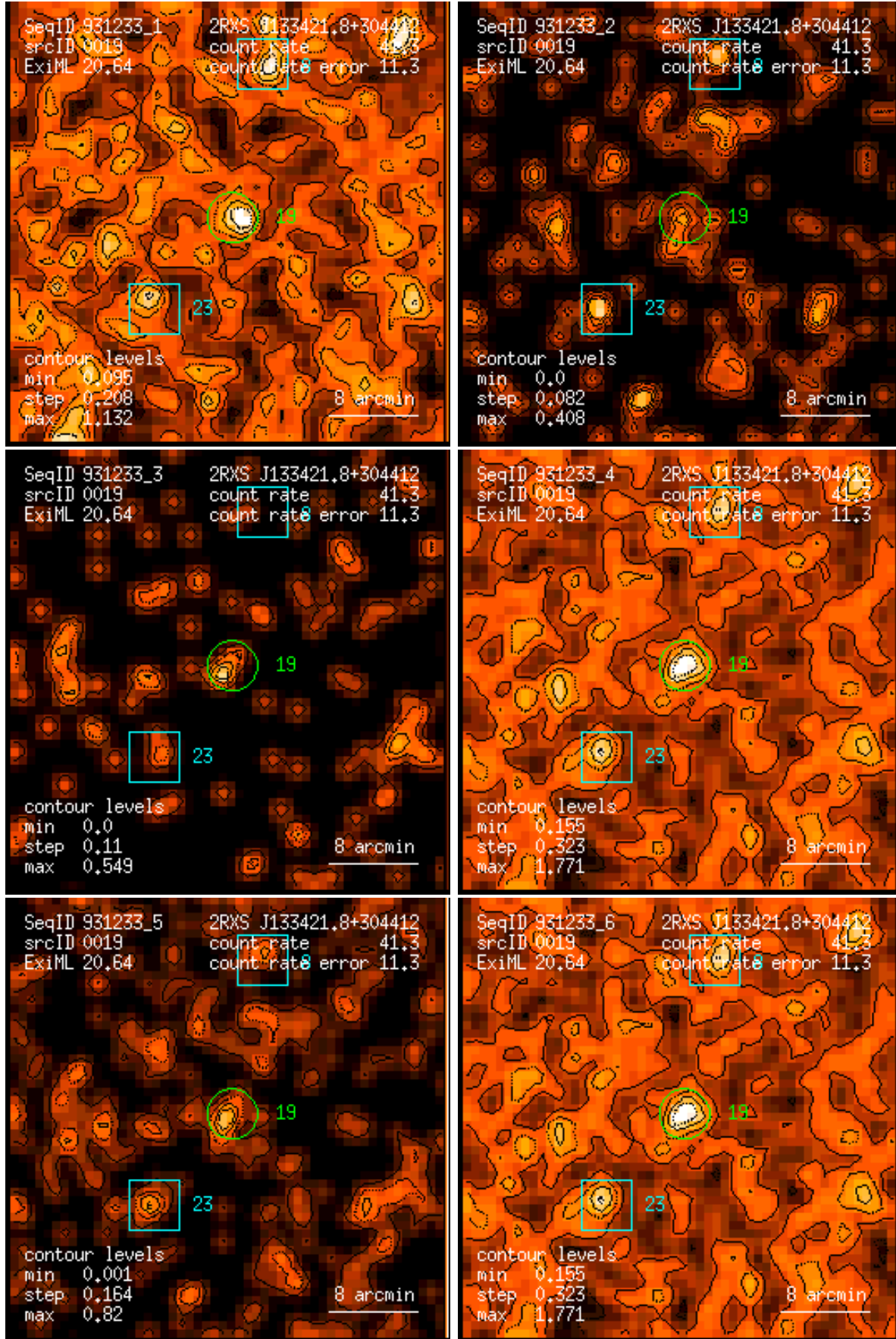
Figure 19: RASS 931233: detection 0019: band rate images, Gaussian filter: (1) PSPC channels 11 – 41, (2) 52 – 90, (3) 91 – 201, (4) 11 – 235, (5) 52 – 201, (6) 11 – 201. Broad band rates in counts/ks. Band rate contour levels in counts/ks/arcmin 2 .
