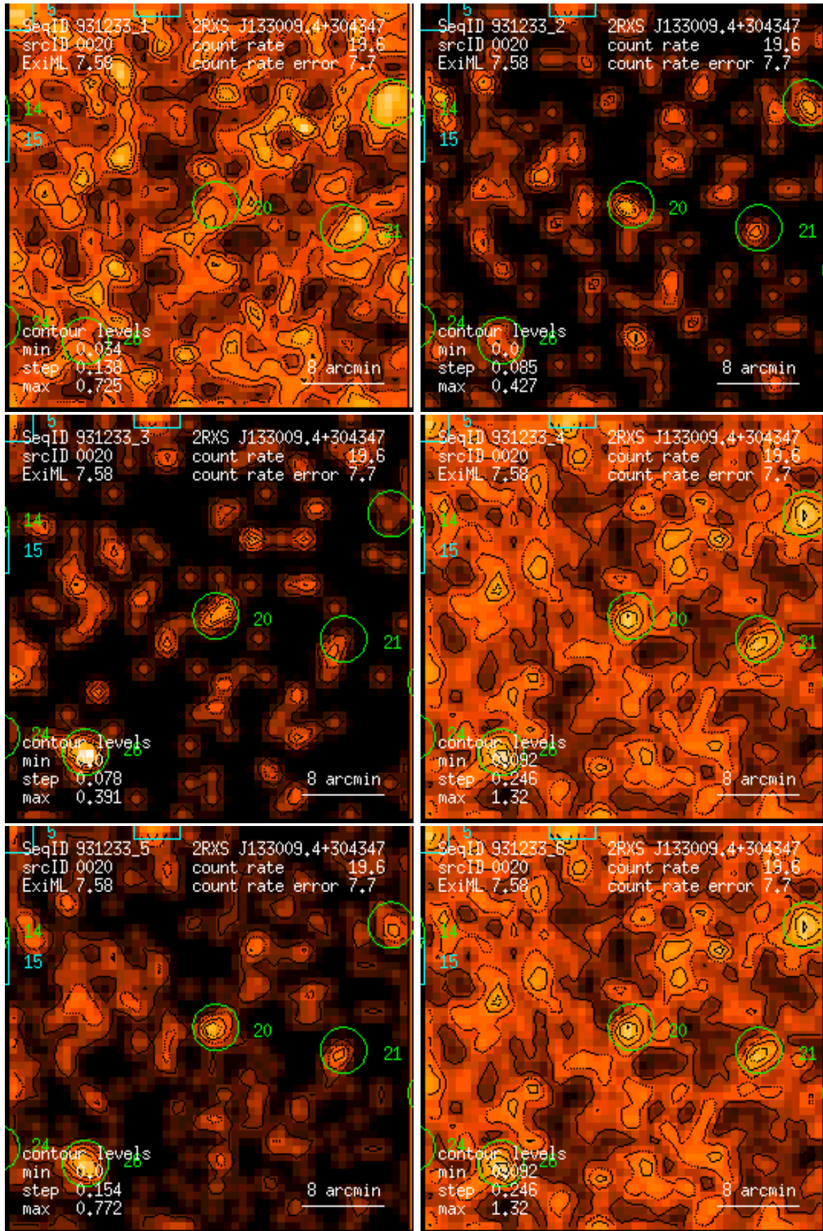
Figure 20: RASS 931233: detection 0020: band rate images, Gaussian filter: (1) PSPC channels 11 – 41, (2) 52 – 90, (3) 91 – 201, (4) 11 – 235, (5) 52 – 201, (6) 11 – 201. Broad band rates in counts/ks. Band rate contour levels in counts/ks/arcmin 2 .
