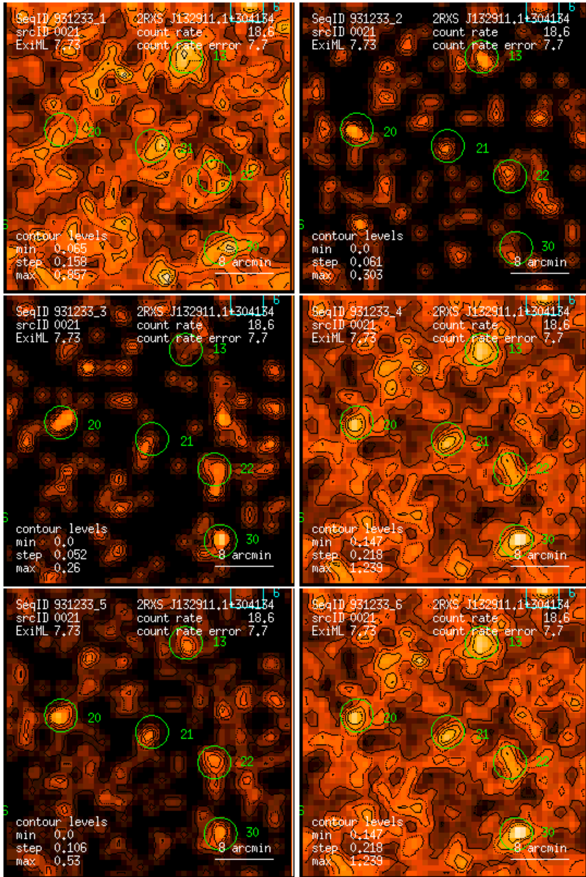
Figure 21: RASS 931233: detection 0021: band rate images, Gaussian filter: (1) PSPC channels 11 – 41, (2) 52 – 90, (3) 91 – 201, (4) 11 – 235, (5) 52 – 201, (6) 11 – 201. Broad band rates in counts/ks. Band rate contour levels in counts/ks/arcmin 2 .
