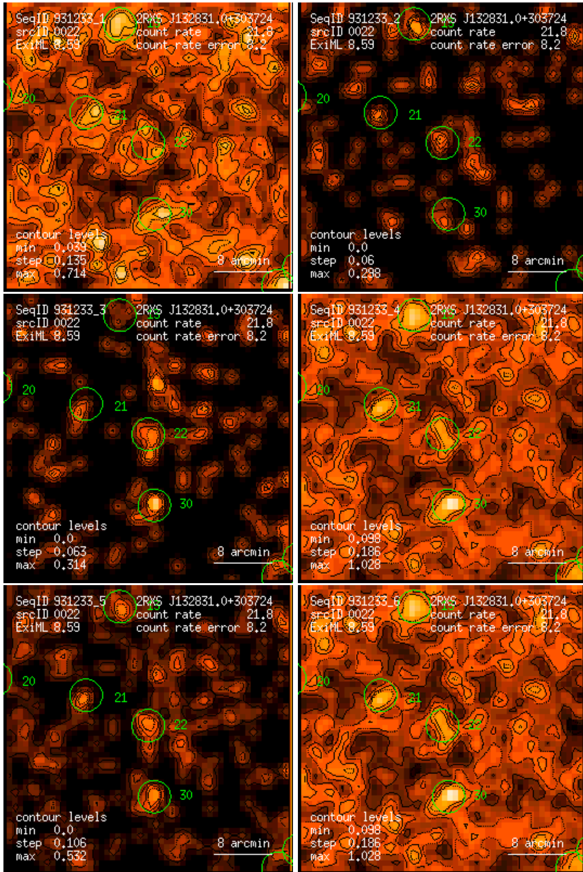
Figure 22: RASS 931233: detection 0022: band rate images, Gaussian filter: (1) PSPC channels 11 – 41, (2) 52 – 90, (3) 91 – 201, (4) 11 – 235, (5) 52 – 201, (6) 11 – 201. Broad band rates in counts/ks. Band rate contour levels in counts/ks/arcmin 2 .
