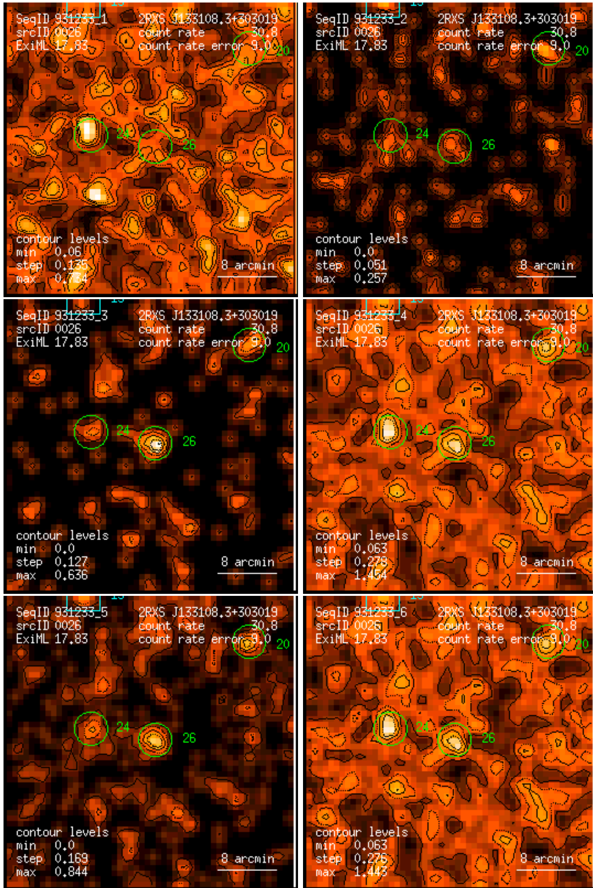
Figure 26: RASS 931233: detection 0026: band rate images, Gaussian filter: (1) PSPC channels 11 – 41, (2) 52 – 90, (3) 91 – 201, (4) 11 – 235, (5) 52 – 201, (6) 11 – 201. Broad band rates in counts/ks. Band rate contour levels in counts/ks/arcmin 2 .
