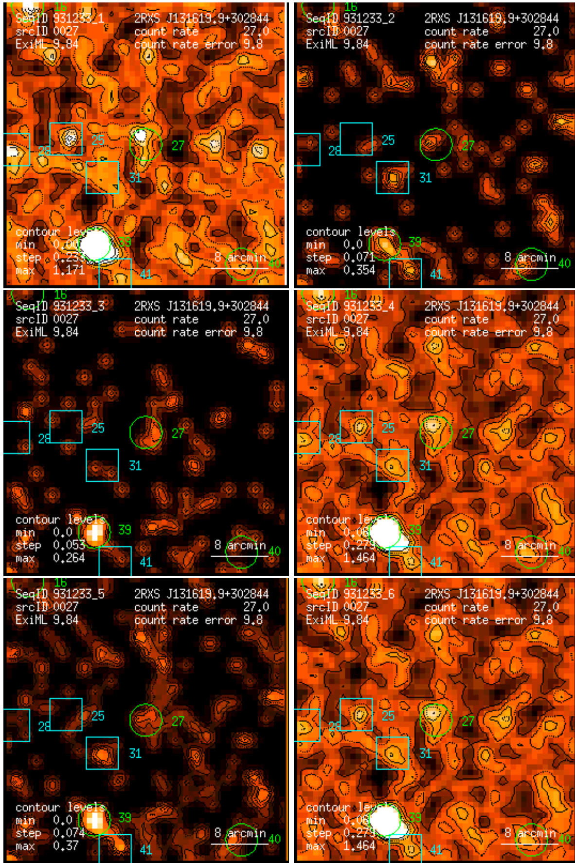
Figure 27: RASS 931233: detection 0027: band rate images, Gaussian filter: (1) PSPC channels 11 – 41, (2) 52 – 90, (3) 91 – 201, (4) 11 – 235, (5) 52 – 201, (6) 11 – 201. Broad band rates in counts/ks. Band rate contour levels in counts/ks/arcmin 2 .
