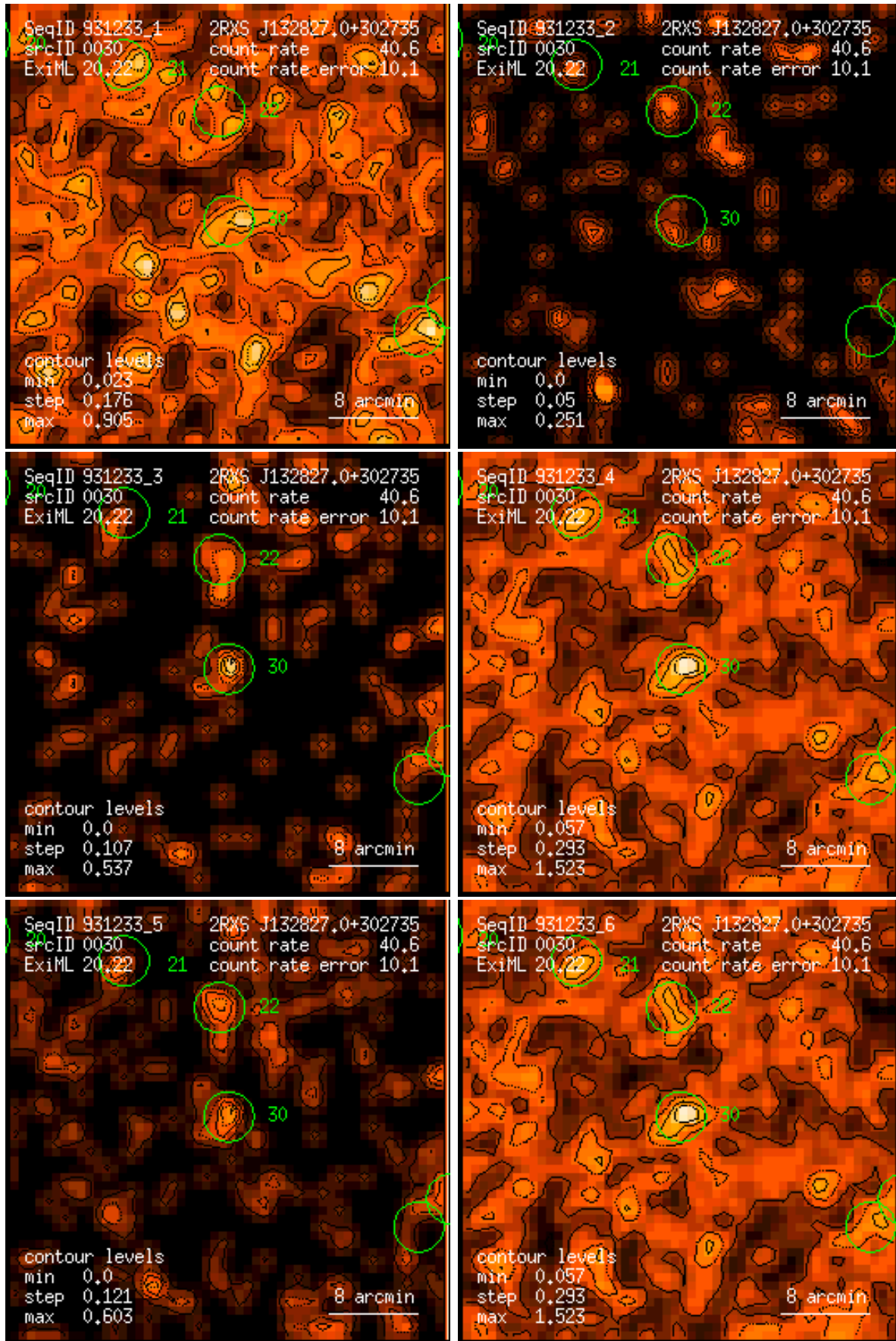
Figure 30: RASS 931233: detection 0030: band rate images, Gaussian filter: (1) PSPC channels 11 – 41, (2) 52 – 90, (3) 91 – 201, (4) 11 – 235, (5) 52 – 201, (6) 11 – 201. Broad band rates in counts/ks. Band rate contour levels in counts/ks/arcmin 2 .
