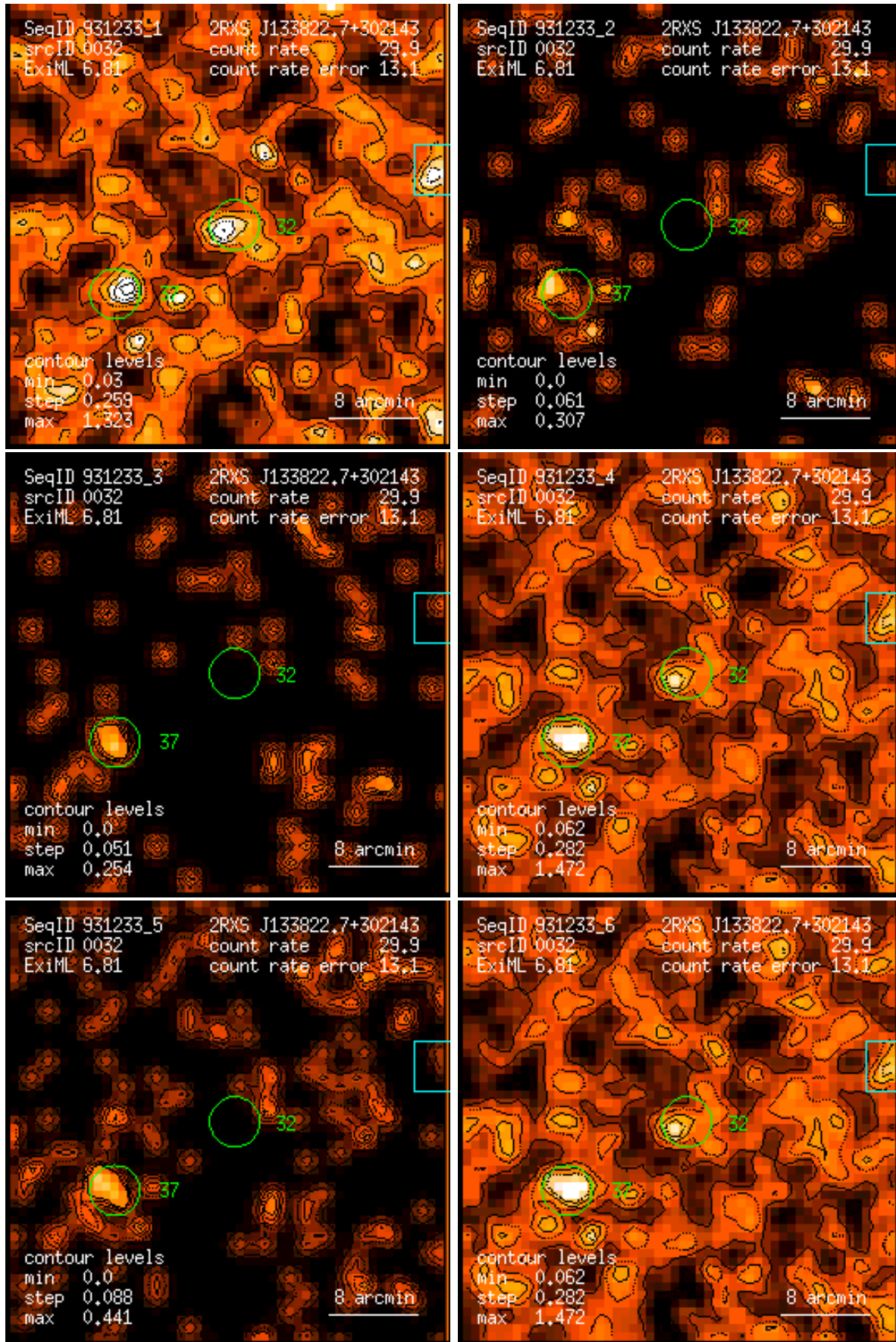
Figure 32: RASS 931233: detection 0032: band rate images, Gaussian filter: (1) PSPC channels 11 – 41, (2) 52 – 90, (3) 91 – 201, (4) 11 – 235, (5) 52 – 201, (6) 11 – 201. Broad band rates in counts/ks. Band rate contour levels in counts/ks/arcmin 2 .
