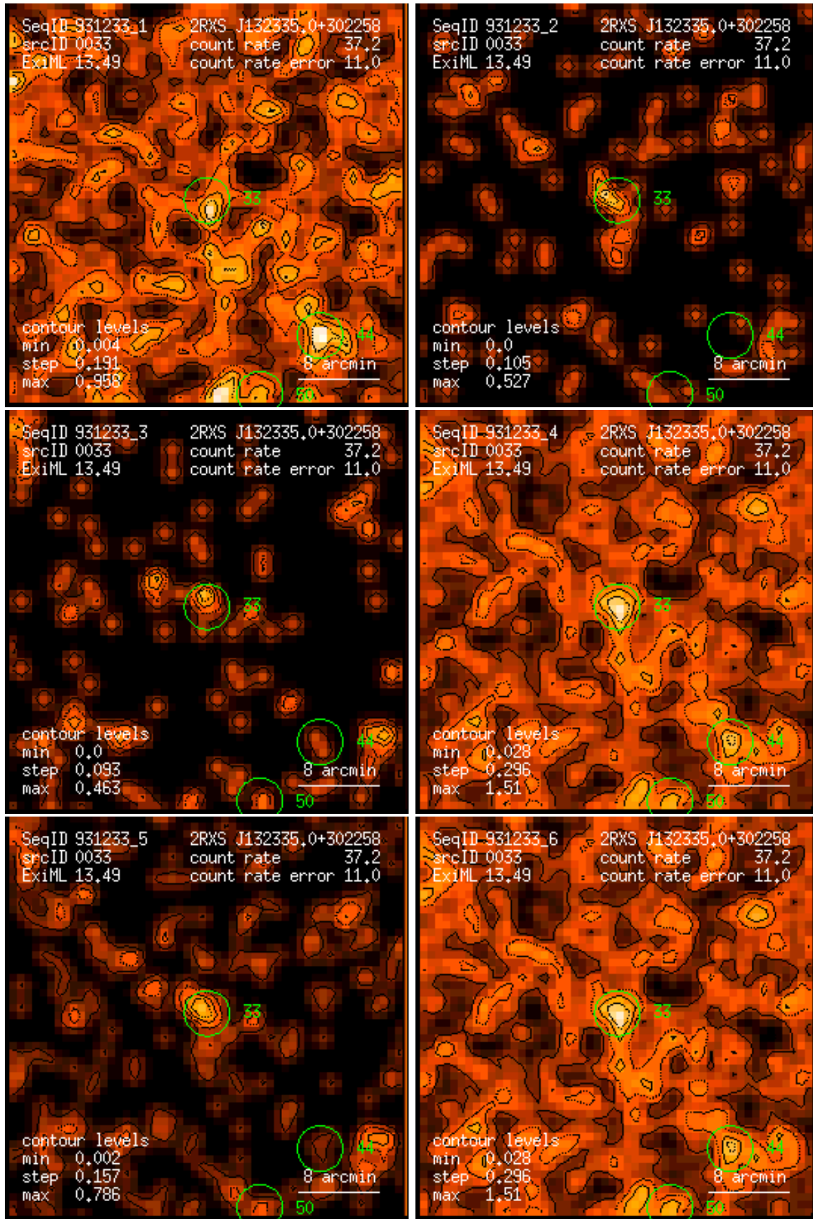
Figure 33: RASS 931233: detection 0033: band rate images, Gaussian filter: (1) PSPC channels 11 – 41, (2) 52 – 90, (3) 91 – 201, (4) 11 – 235, (5) 52 – 201, (6) 11 – 201. Broad band rates in counts/ks. Band rate contour levels in counts/ks/arcmin 2 .
