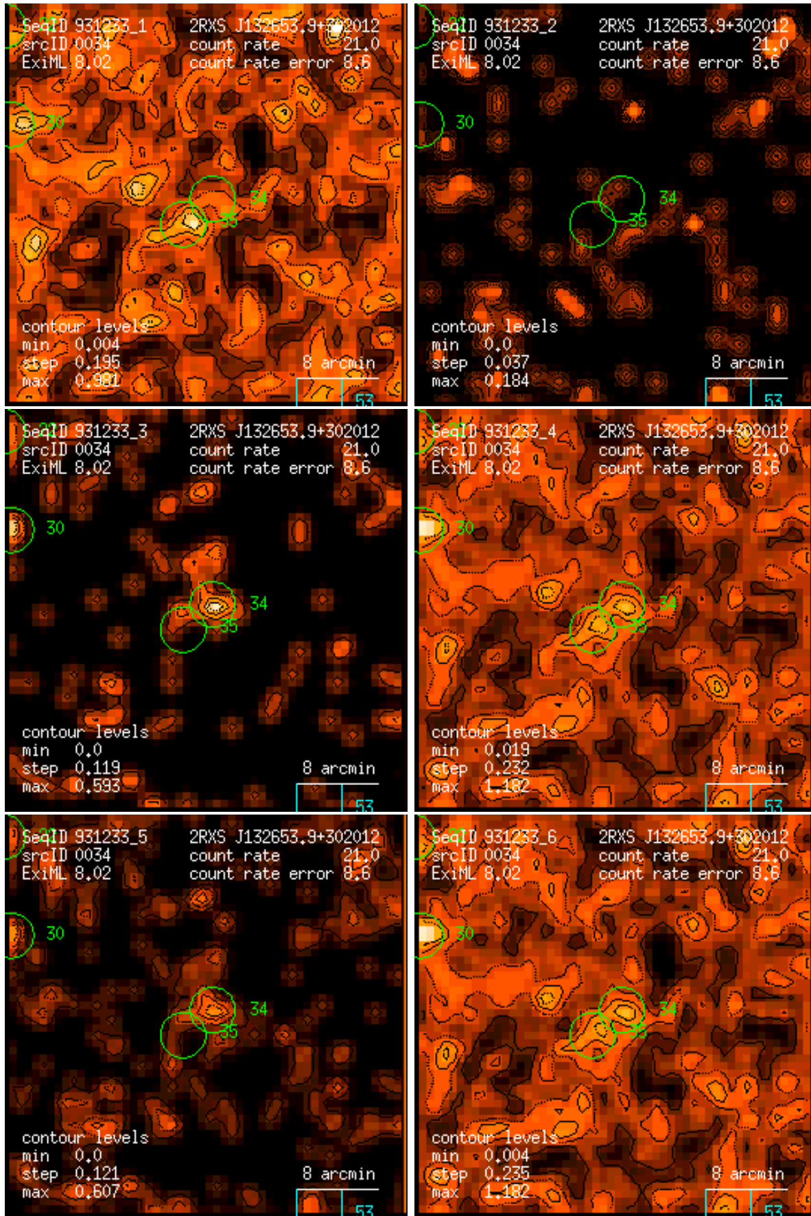
Figure 34: RASS 931233: detection 0034: band rate images, Gaussian filter: (1) PSPC channels 11 – 41, (2) 52 – 90, (3) 91 – 201, (4) 11 – 235, (5) 52 – 201, (6) 11 – 201. Broad band rates in counts/ks. Band rate contour levels in counts/ks/arcmin 2 .
