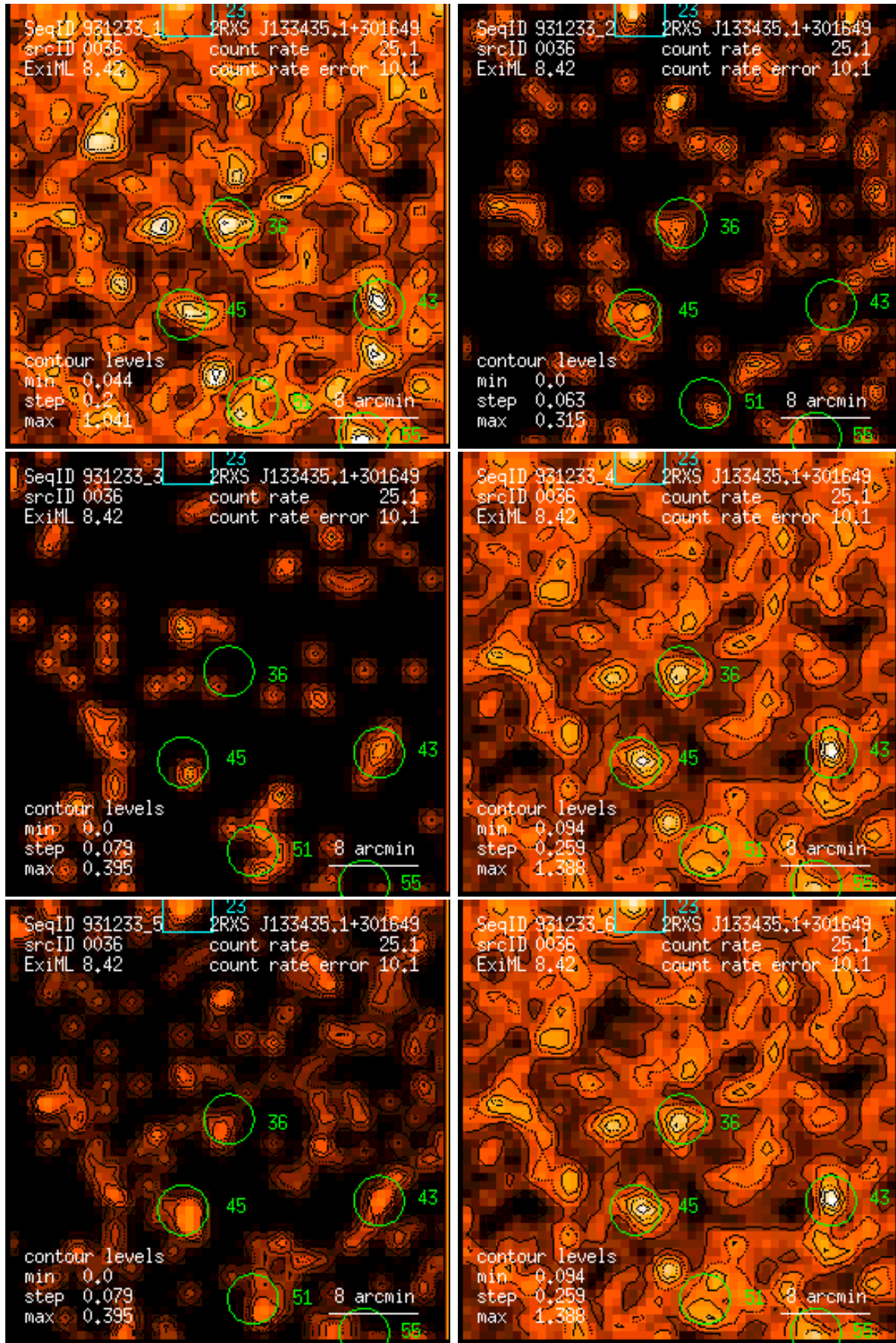
Figure 36: RASS 931233: detection 0036: band rate images, Gaussian filter: (1) PSPC channels 11 – 41, (2) 52 – 90, (3) 91 – 201, (4) 11 – 235, (5) 52 – 201, (6) 11 – 201. Broad band rates in counts/ks. Band rate contour levels in counts/ks/arcmin 2 .
