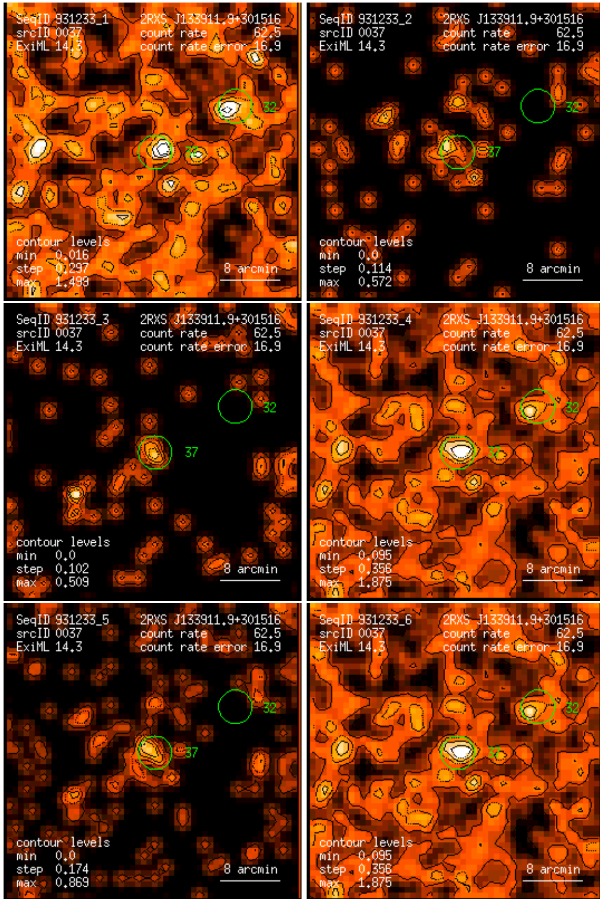
Figure 37: RASS 931233: detection 0037: band rate images, Gaussian filter: (1) PSPC channels 11 – 41, (2) 52 – 90, (3) 91 – 201, (4) 11 – 235, (5) 52 – 201, (6) 11 – 201. Broad band rates in counts/ks. Band rate contour levels in counts/ks/arcmin 2 .
