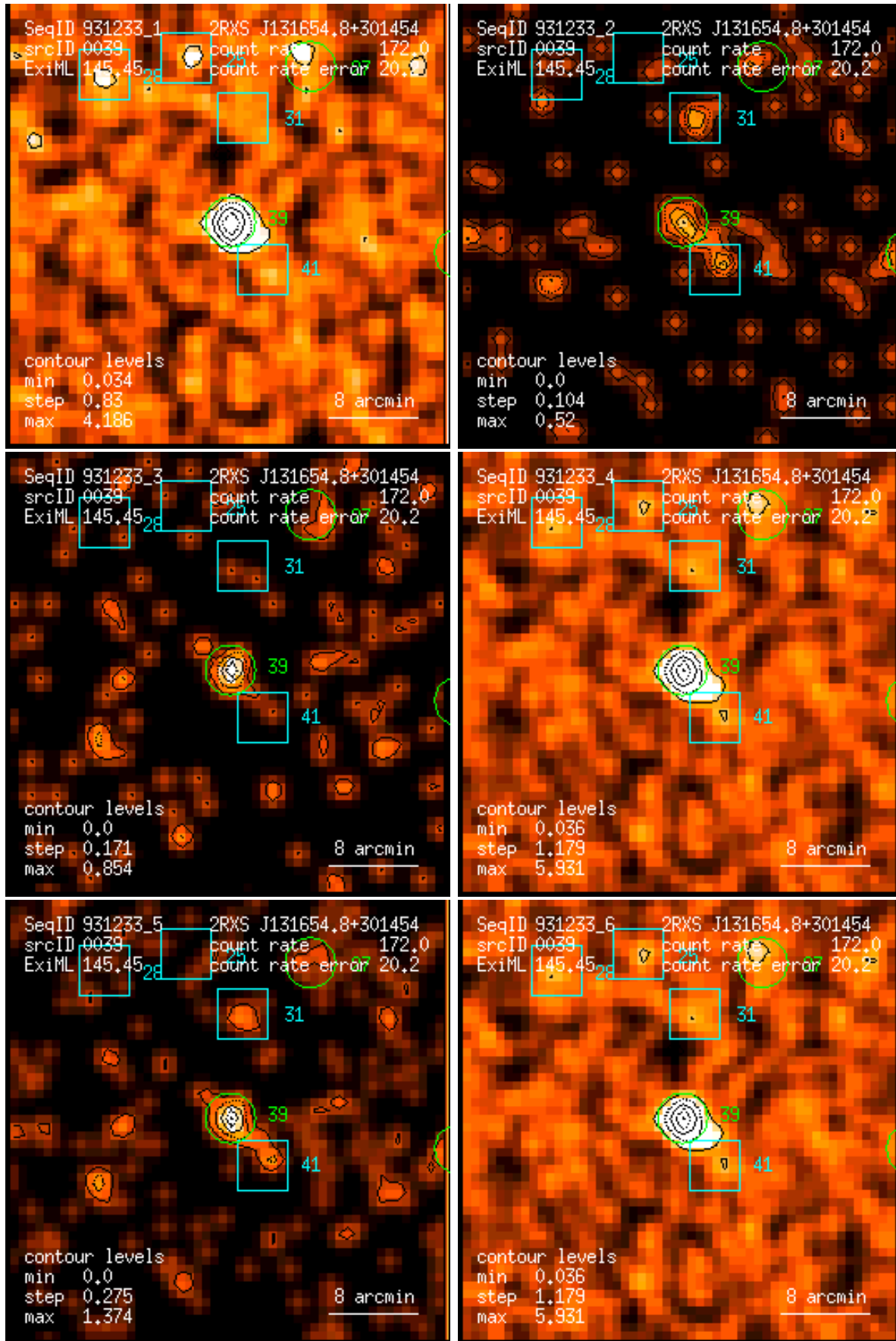
Figure 39: RASS 931233: detection 0039: band rate images, Gaussian filter: (1) PSPC channels 11 – 41, (2) 52 – 90, (3) 91 – 201, (4) 11 – 235, (5) 52 – 201, (6) 11 – 201. Broad band rates in counts/ks. Band rate contour levels in counts/ks/arcmin 2 .
