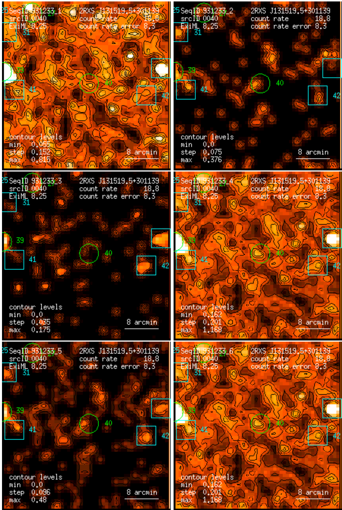
Figure 40: RASS 931233: detection 0040: band rate images, Gaussian filter: (1) PSPC channels 11 – 41, (2) 52 – 90, (3) 91 – 201, (4) 11 – 235, (5) 52 – 201, (6) 11 – 201. Broad band rates in counts/ks. Band rate contour levels in counts/ks/arcmin 2 .
