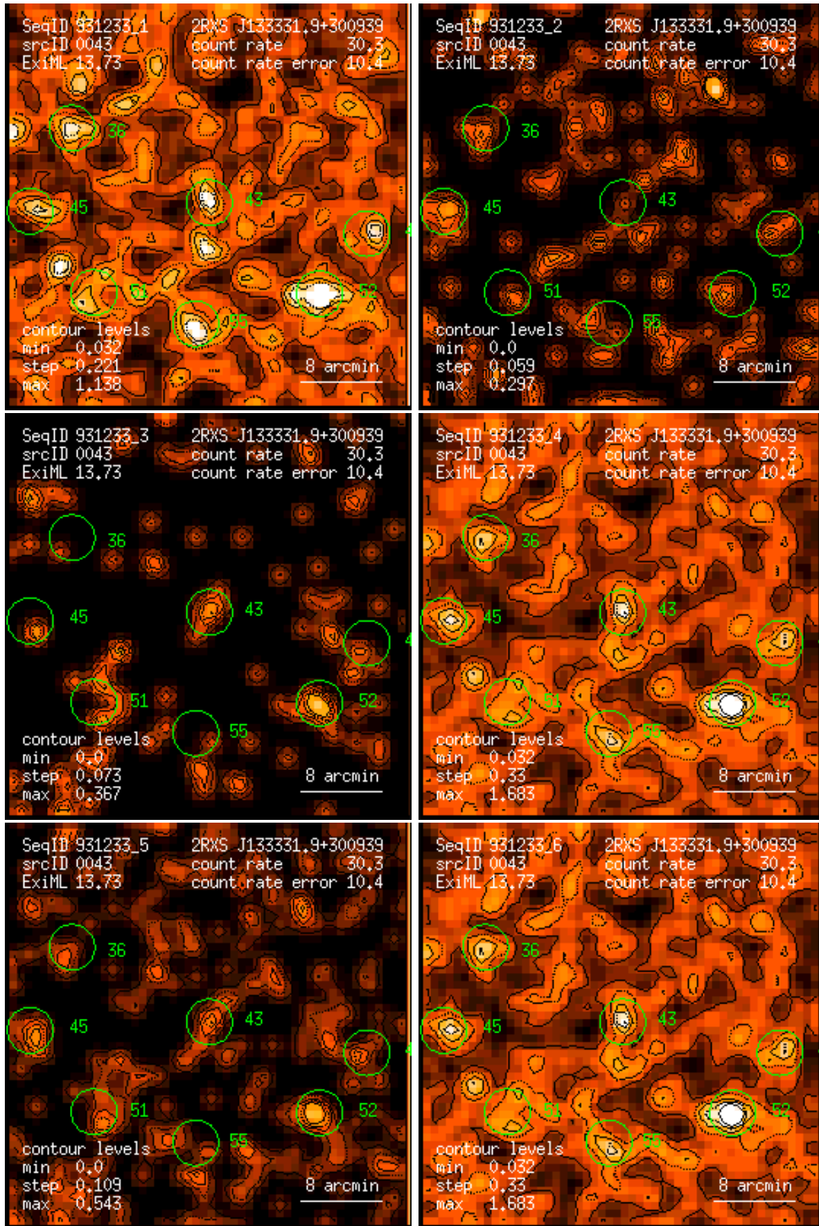
Figure 43: RASS 931233: detection 0043: band rate images, Gaussian filter: (1) PSPC channels 11 – 41, (2) 52 – 90, (3) 91 – 201, (4) 11 – 235, (5) 52 – 201, (6) 11 – 201. Broad band rates in counts/ks. Band rate contour levels in counts/ks/arcmin 2 .
