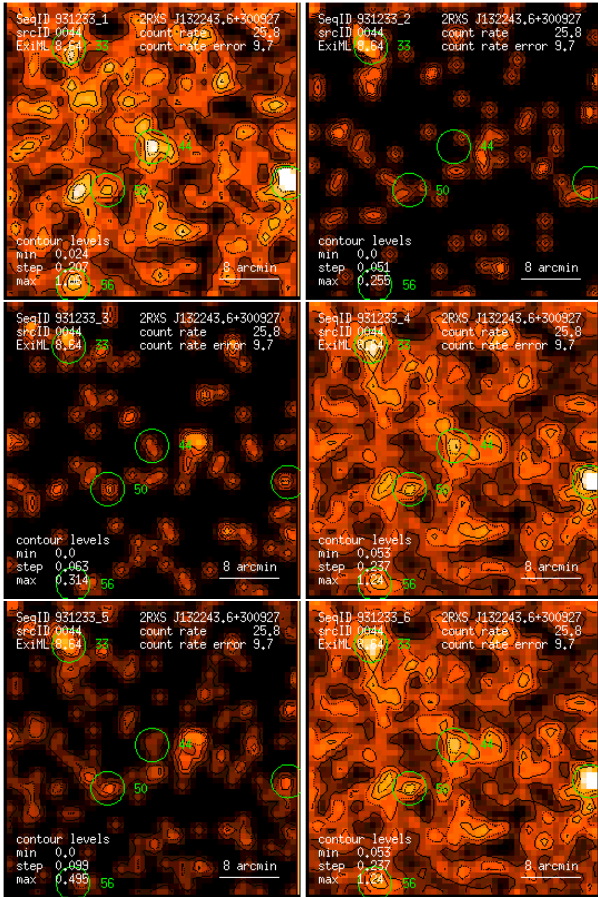
Figure 44: RASS 931233: detection 0044: band rate images, Gaussian filter: (1) PSPC channels 11 – 41, (2) 52 – 90, (3) 91 – 201, (4) 11 – 235, (5) 52 – 201, (6) 11 – 201. Broad band rates in counts/ks. Band rate contour levels in counts/ks/arcmin 2 .
