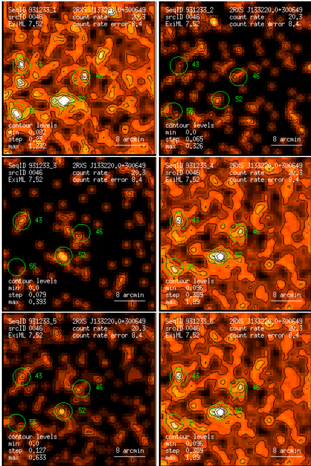
Figure 46: RASS 931233: detection 0046: band rate images, Gaussian filter: (1) PSPC channels 11 – 41, (2) 52 – 90, (3) 91 – 201, (4) 11 – 235, (5) 52 – 201, (6) 11 – 201. Broad band rates in counts/ks. Band rate contour levels in counts/ks/arcmin 2 .
