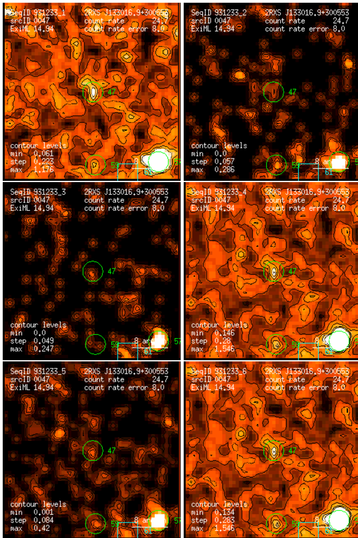
Figure 47: RASS 931233: detection 0047: band rate images, Gaussian filter: (1) PSPC channels 11 – 41, (2) 52 – 90, (3) 91 – 201, (4) 11 – 235, (5) 52 – 201, (6) 11 – 201. Broad band rates in counts/ks. Band rate contour levels in counts/ks/arcmin 2 .
