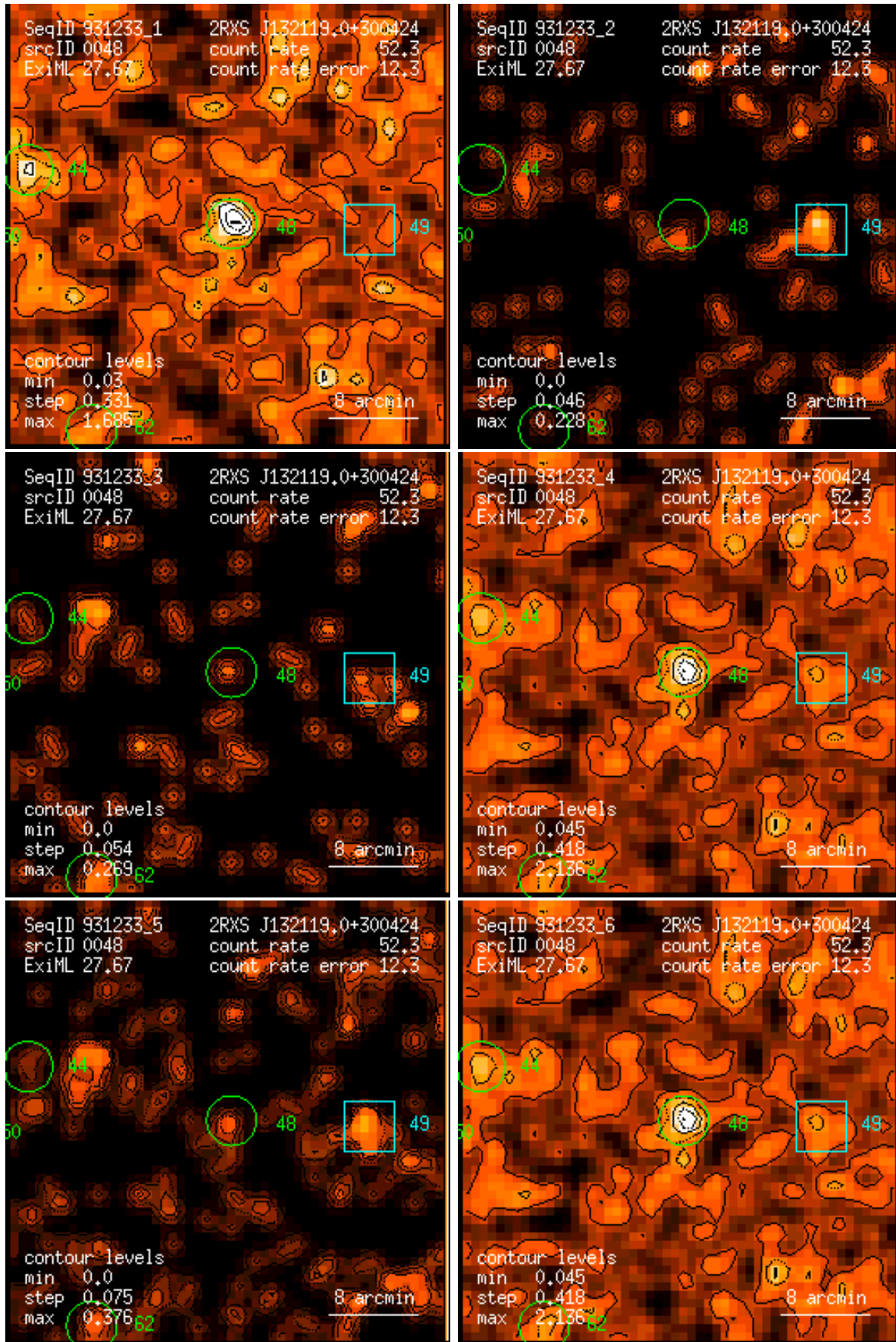
Figure 48: RASS 931233: detection 0048: band rate images, Gaussian filter: (1) PSPC channels 11 – 41, (2) 52 – 90, (3) 91 – 201, (4) 11 – 235, (5) 52 – 201, (6) 11 – 201. Broad band rates in counts/ks. Band rate contour levels in counts/ks/arcmin 2 .
