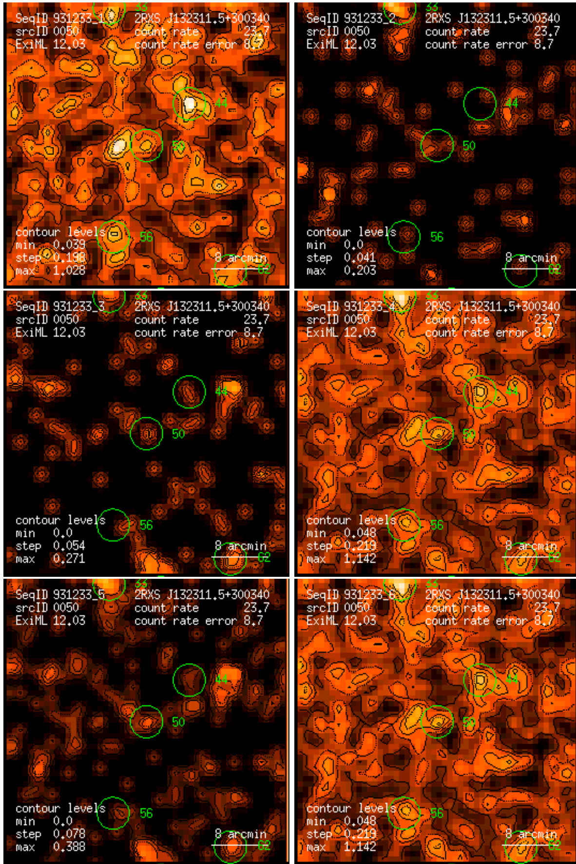
Figure 50: RASS 931233: detection 0050: band rate images, Gaussian filter: (1) PSPC channels 11 – 41, (2) 52 – 90, (3) 91 – 201, (4) 11 – 235, (5) 52 – 201, (6) 11 – 201. Broad band rates in counts/ks. Band rate contour levels in counts/ks/arcmin 2 .
