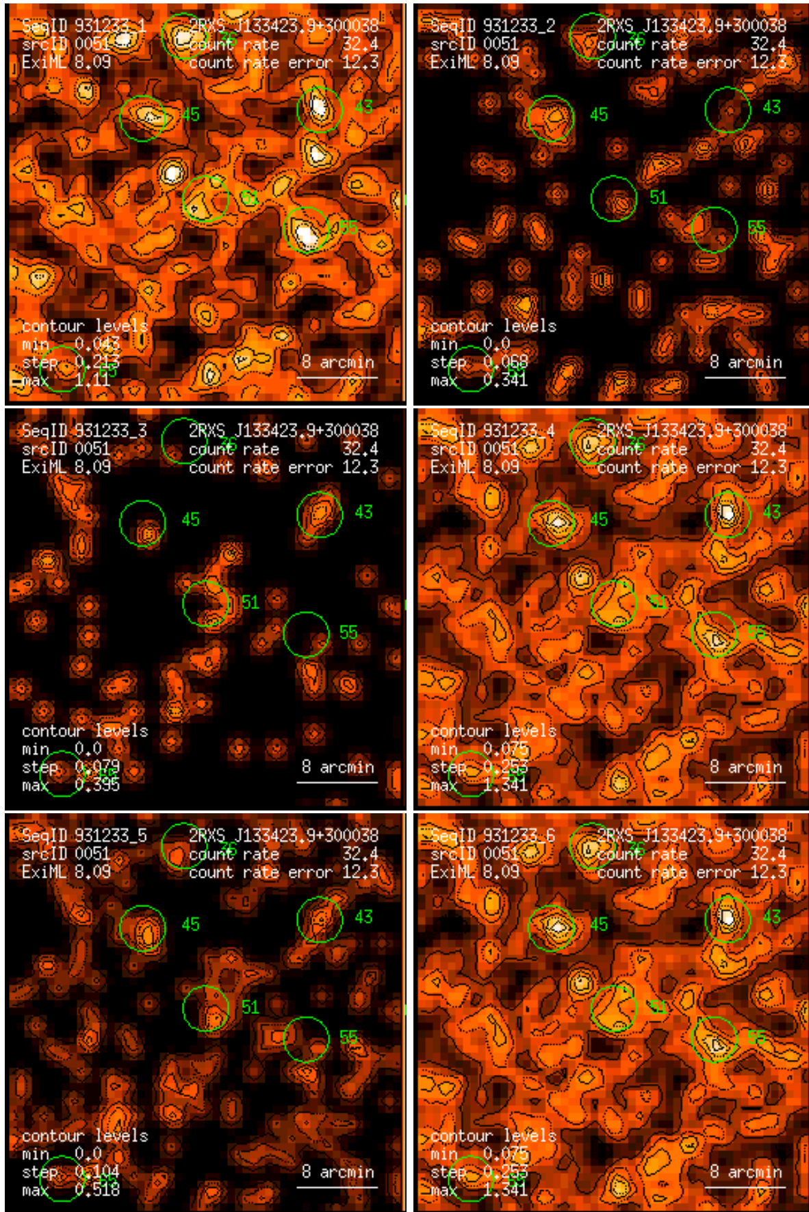
Figure 51: RASS 931233: detection 0051: band rate images, Gaussian filter: (1) PSPC channels 11 – 41, (2) 52 – 90, (3) 91 – 201, (4) 11 – 235, (5) 52 – 201, (6) 11 – 201. Broad band rates in counts/ks. Band rate contour levels in counts/ks/arcmin 2 .
