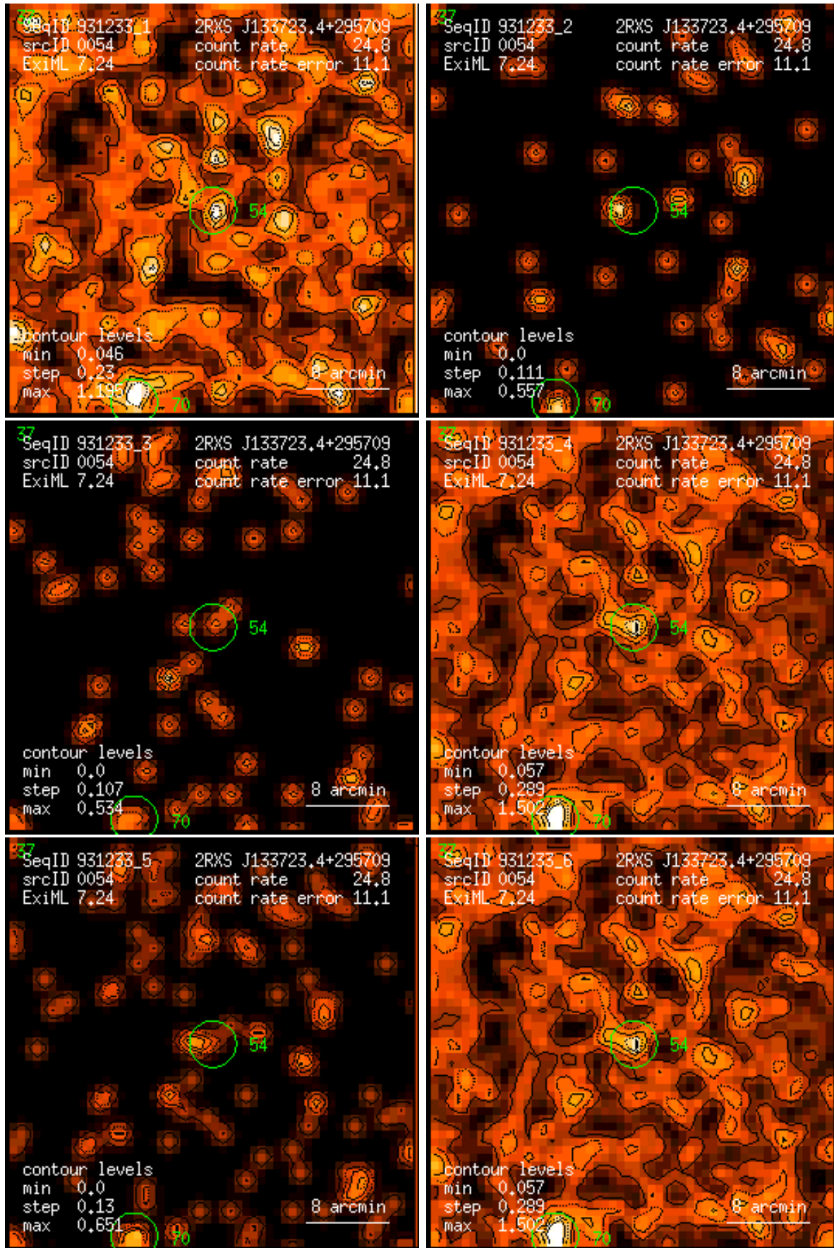
Figure 54: RASS 931233: detection 0054: band rate images, Gaussian filter: (1) PSPC channels 11 – 41, (2) 52 – 90, (3) 91 – 201, (4) 11 – 235, (5) 52 – 201, (6) 11 – 201. Broad band rates in counts/ks. Band rate contour levels in counts/ks/arcmin 2 .
