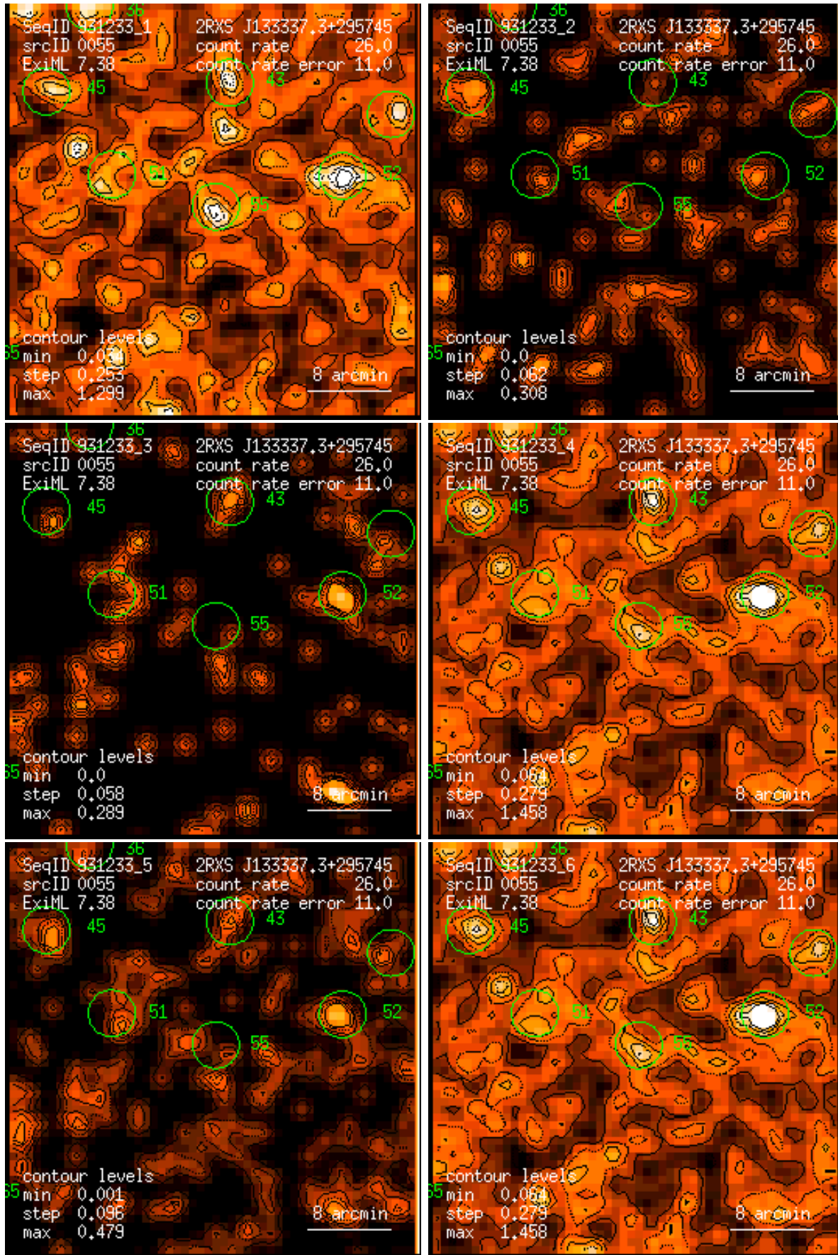
Figure 55: RASS 931233: detection 0055: band rate images, Gaussian filter: (1) PSPC channels 11 – 41, (2) 52 – 90, (3) 91 – 201, (4) 11 – 235, (5) 52 – 201, (6) 11 – 201. Broad band rates in counts/ks. Band rate contour levels in counts/ks/arcmin 2 .
