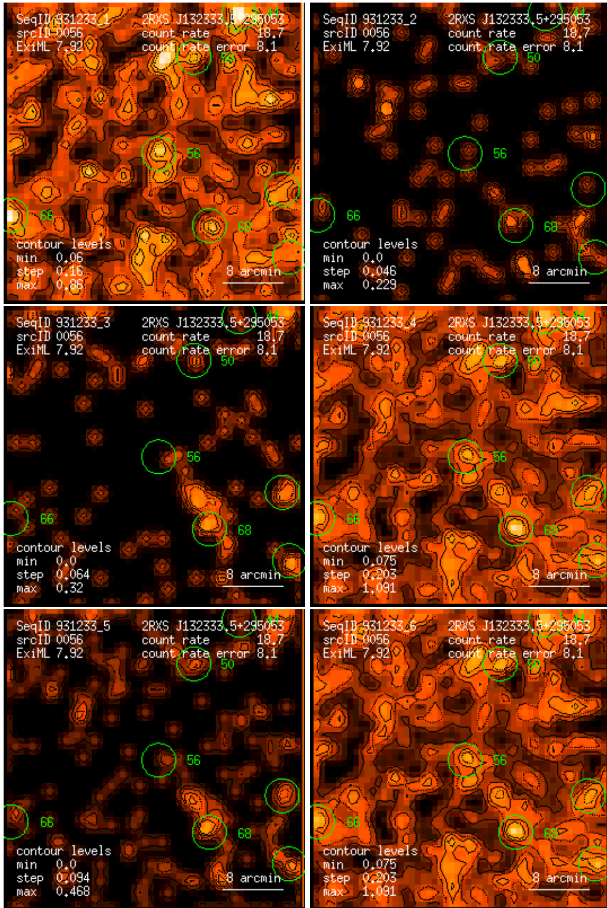
Figure 56: RASS 931233: detection 0056: band rate images, Gaussian filter: (1) PSPC channels 11 – 41, (2) 52 – 90, (3) 91 – 201, (4) 11 – 235, (5) 52 – 201, (6) 11 – 201. Broad band rates in counts/ks. Band rate contour levels in counts/ks/arcmin 2 .
