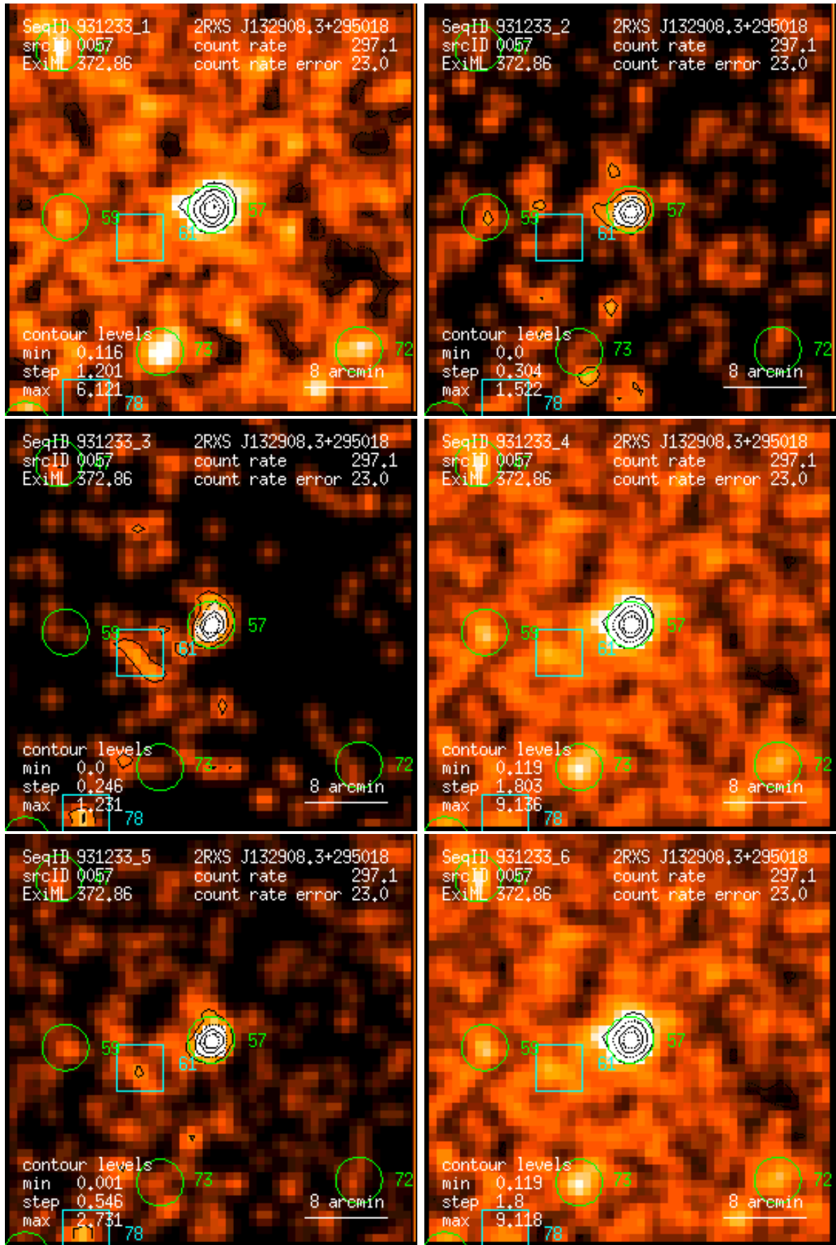
Figure 57: RASS 931233: detection 0057: band rate images, Gaussian filter: (1) PSPC channels 11 – 41, (2) 52 – 90, (3) 91 – 201, (4) 11 – 235, (5) 52 – 201, (6) 11 – 201. Broad band rates in counts/ks. Band rate contour levels in counts/ks/arcmin 2 .
