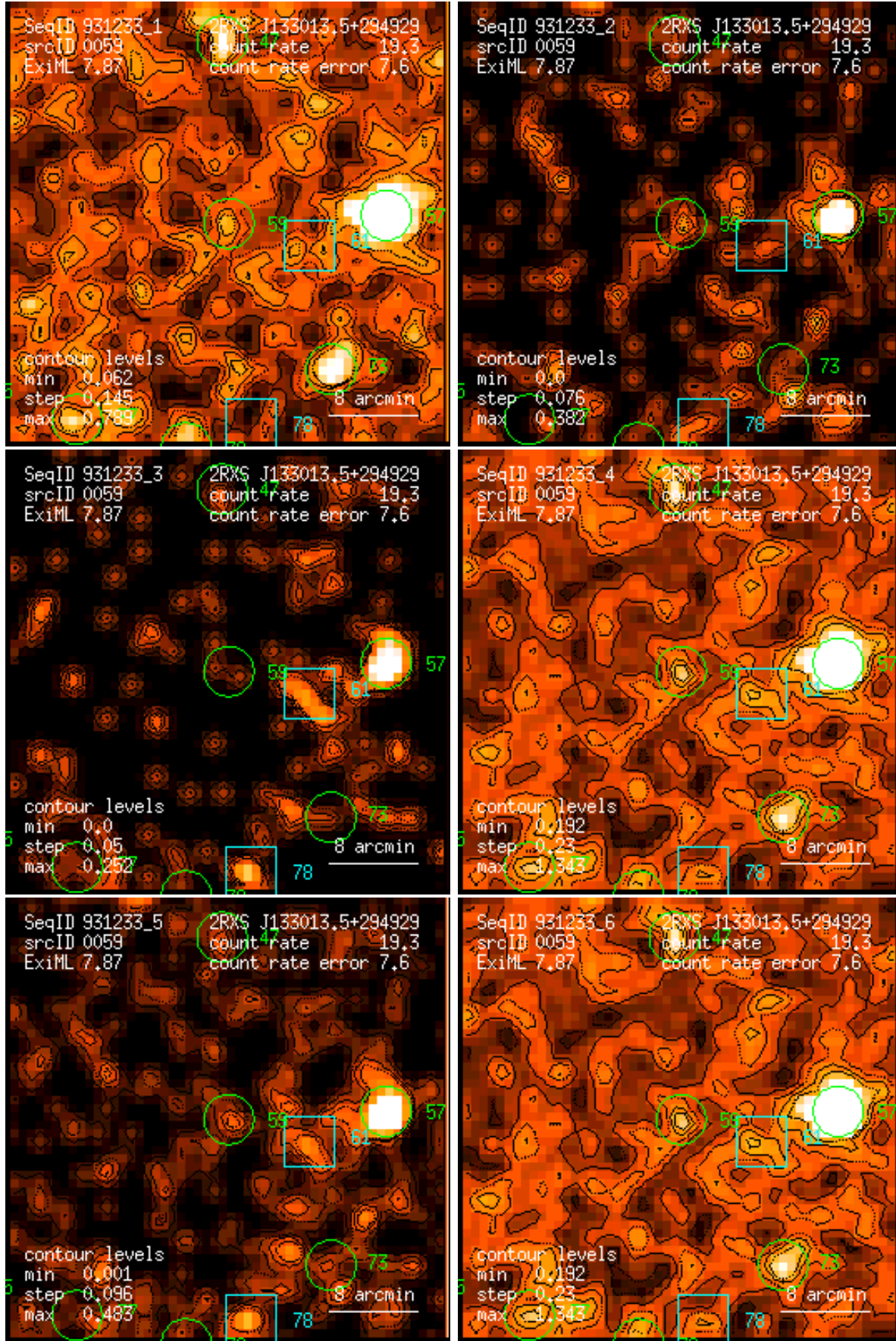
Figure 59: RASS 931233: detection 0059: band rate images, Gaussian filter: (1) PSPC channels 11 – 41, (2) 52 – 90, (3) 91 – 201, (4) 11 – 235, (5) 52 – 201, (6) 11 – 201. Broad band rates in counts/ks. Band rate contour levels in counts/ks/arcmin 2 .
