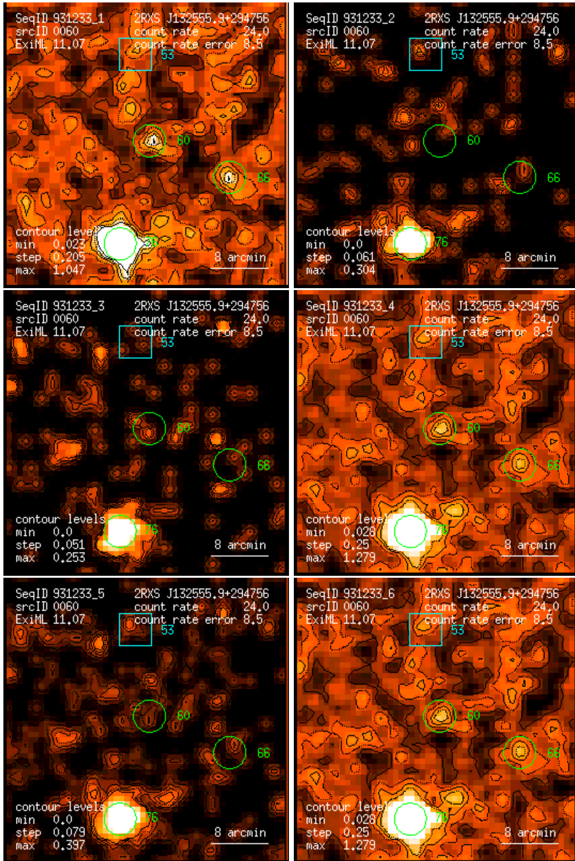
Figure 60: RASS 931233: detection 0060: band rate images, Gaussian filter: (1) PSPC channels 11 – 41, (2) 52 – 90, (3) 91 – 201, (4) 11 – 235, (5) 52 – 201, (6) 11 – 201. Broad band rates in counts/ks. Band rate contour levels in counts/ks/arcmin 2 .
