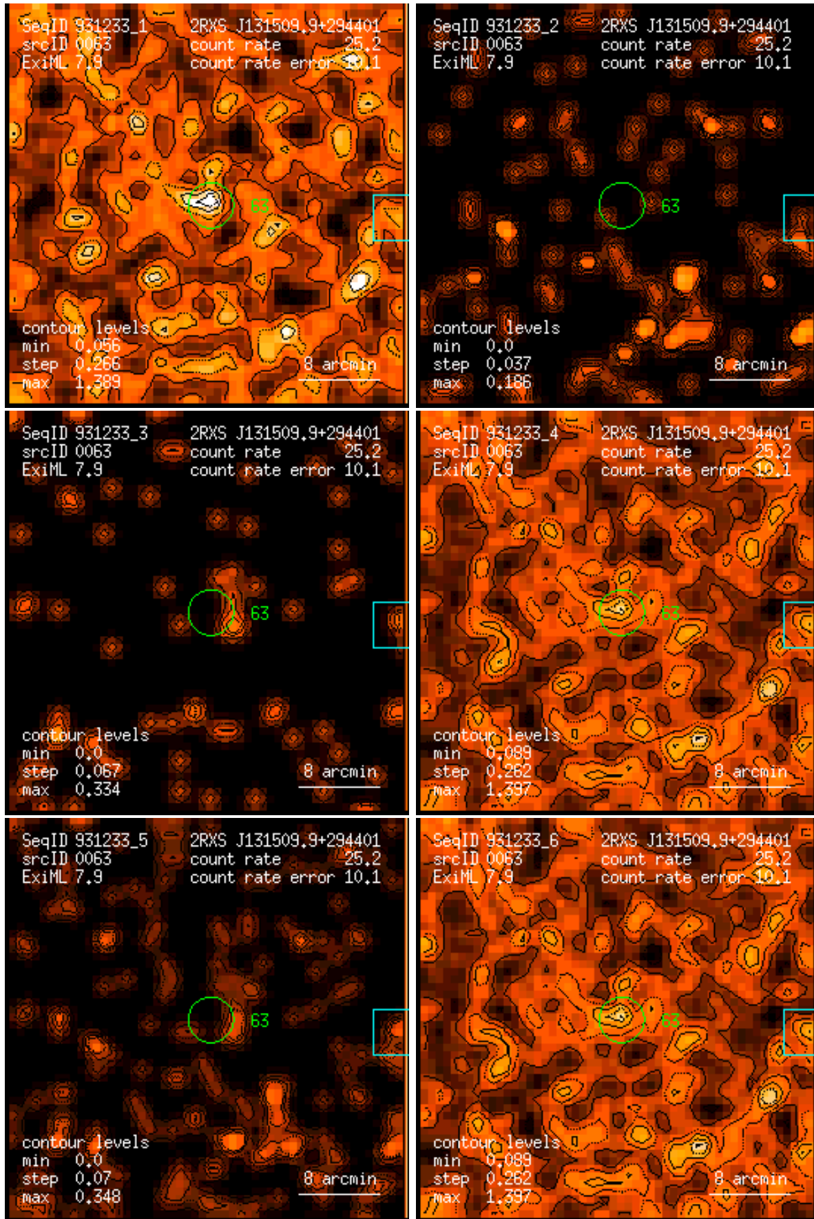
Figure 63: RASS 931233: detection 0063: band rate images, Gaussian filter: (1) PSPC channels 11 – 41, (2) 52 – 90, (3) 91 – 201, (4) 11 – 235, (5) 52 – 201, (6) 11 – 201. Broad band rates in counts/ks. Band rate contour levels in counts/ks/arcmin 2 .
