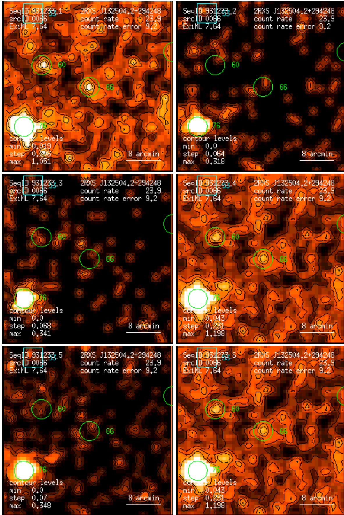
Figure 66: RASS 931233: detection 0066: band rate images, Gaussian filter: (1) PSPC channels 11 – 41, (2) 52 – 90, (3) 91 – 201, (4) 11 – 235, (5) 52 – 201, (6) 11 – 201. Broad band rates in counts/ks. Band rate contour levels in counts/ks/arcmin 2 .
