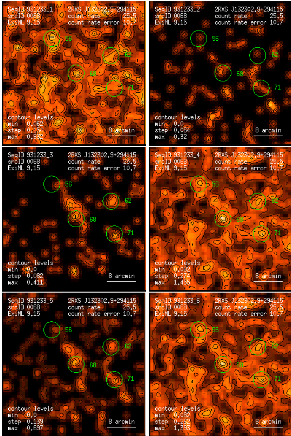
Figure 68: RASS 931233: detection 0068: band rate images, Gaussian filter: (1) PSPC channels 11 – 41, (2) 52 – 90, (3) 91 – 201, (4) 11 – 235, (5) 52 – 201, (6) 11 – 201. Broad band rates in counts/ks. Band rate contour levels in counts/ks/arcmin 2 .
