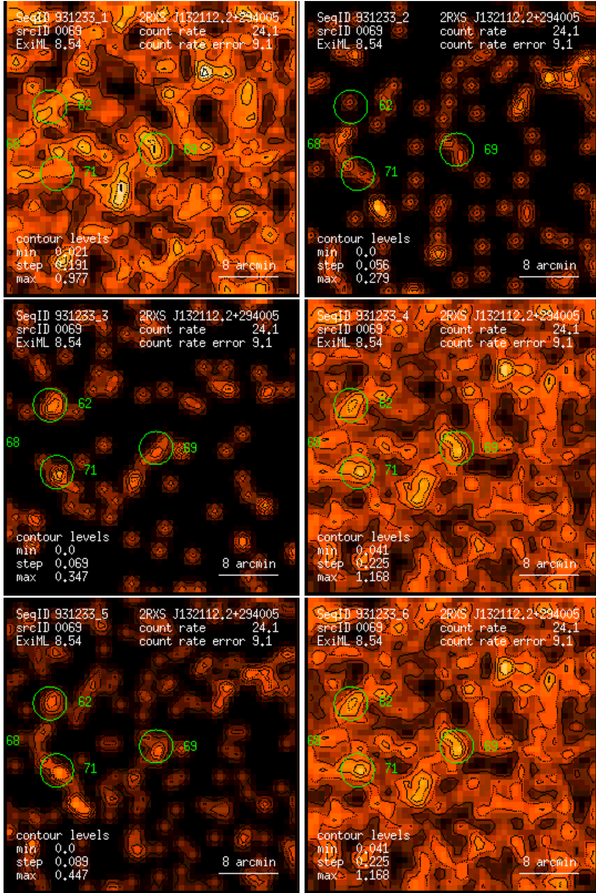
Figure 69: RASS 931233: detection 0069: band rate images, Gaussian filter: (1) PSPC channels 11 – 41, (2) 52 – 90, (3) 91 – 201, (4) 11 – 235, (5) 52 – 201, (6) 11 – 201. Broad band rates in counts/ks. Band rate contour levels in counts/ks/arcmin 2 .
